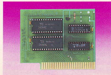
16K Pocket Rocket RAM Card
