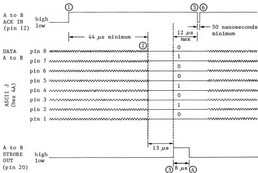
Figure 5-2. Parallel Output Handshake
