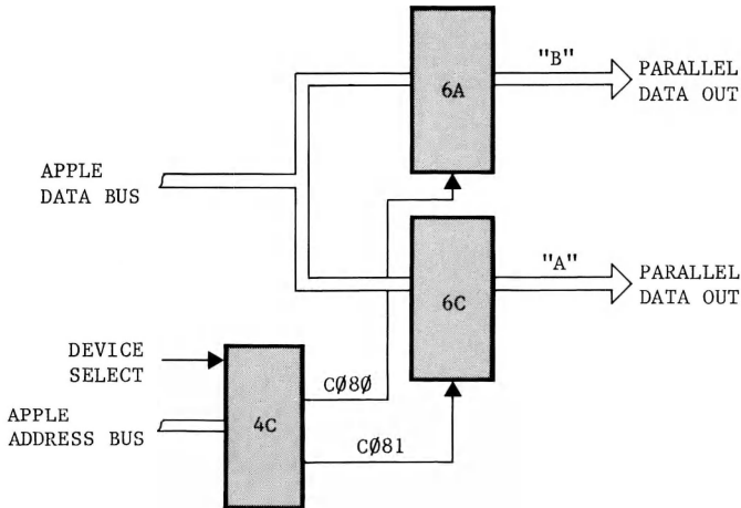
Figure 6-2. Output Port Block Diagram
