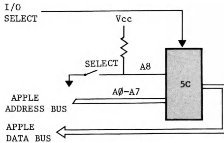
Figure 6-3. Read Only Memory
