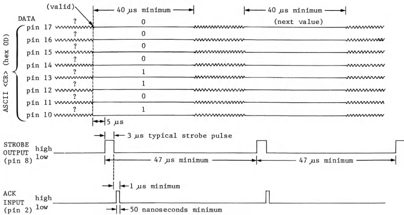
Figure 4-1. The Printer Driver's Handshake
