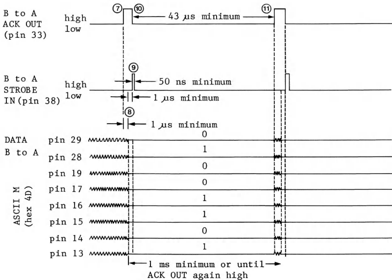
Figure 5-3. Parallel Input Handshake
