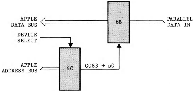
Figure 6-1. Input Port Block Diagram
