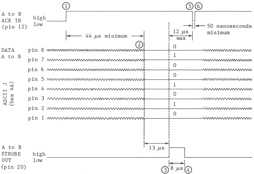
Figure 5-2. Parallel Output Handshake
