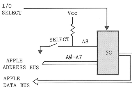
Figure 6-3. Read Only Memory
