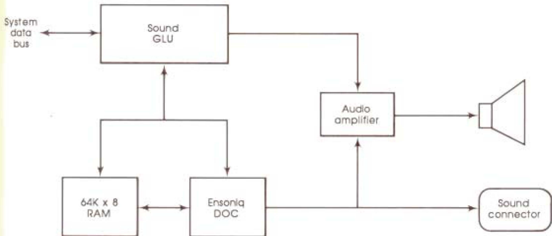
Figure 2-6 Apple IIGS sound system
