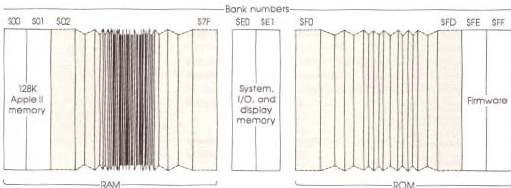
Figure 2-2 Simplified Apple IIGS memory map
