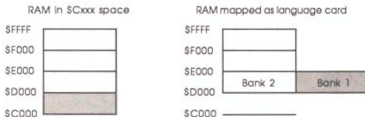
Figure 7-1 Memory map of language-card RAM
