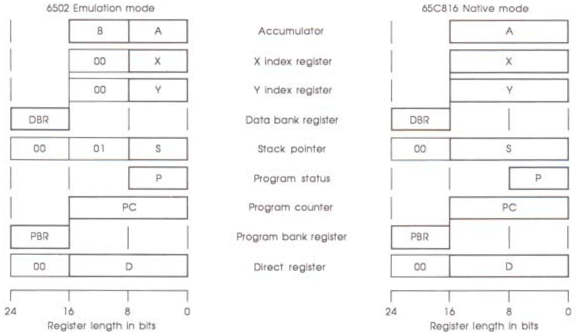
Figure 2-1 65C816 registers
