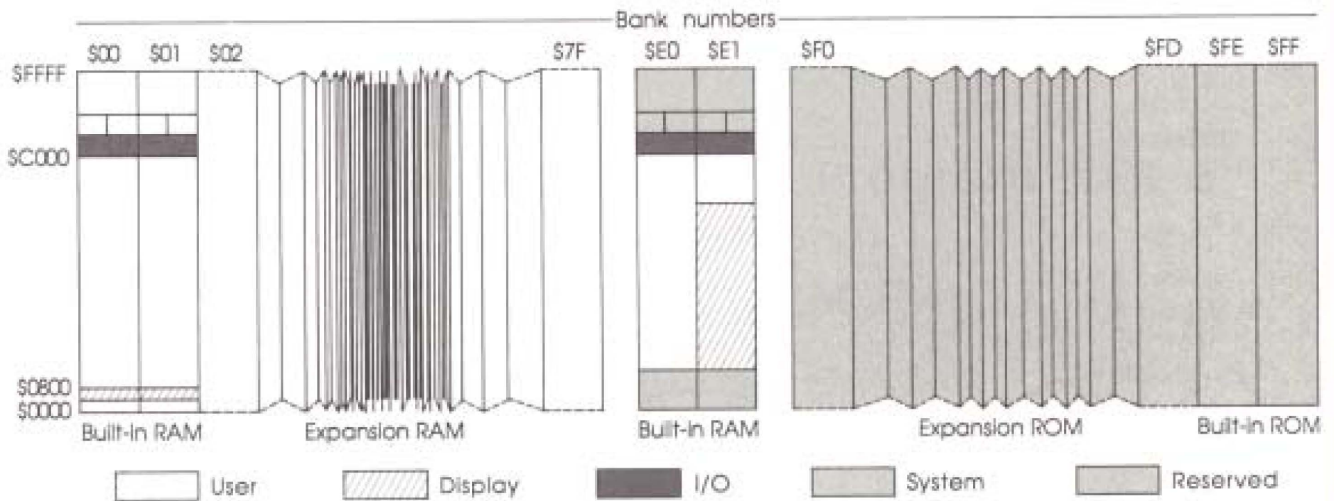
Figure 6-4 Memory map for new Apple IIGS programs
