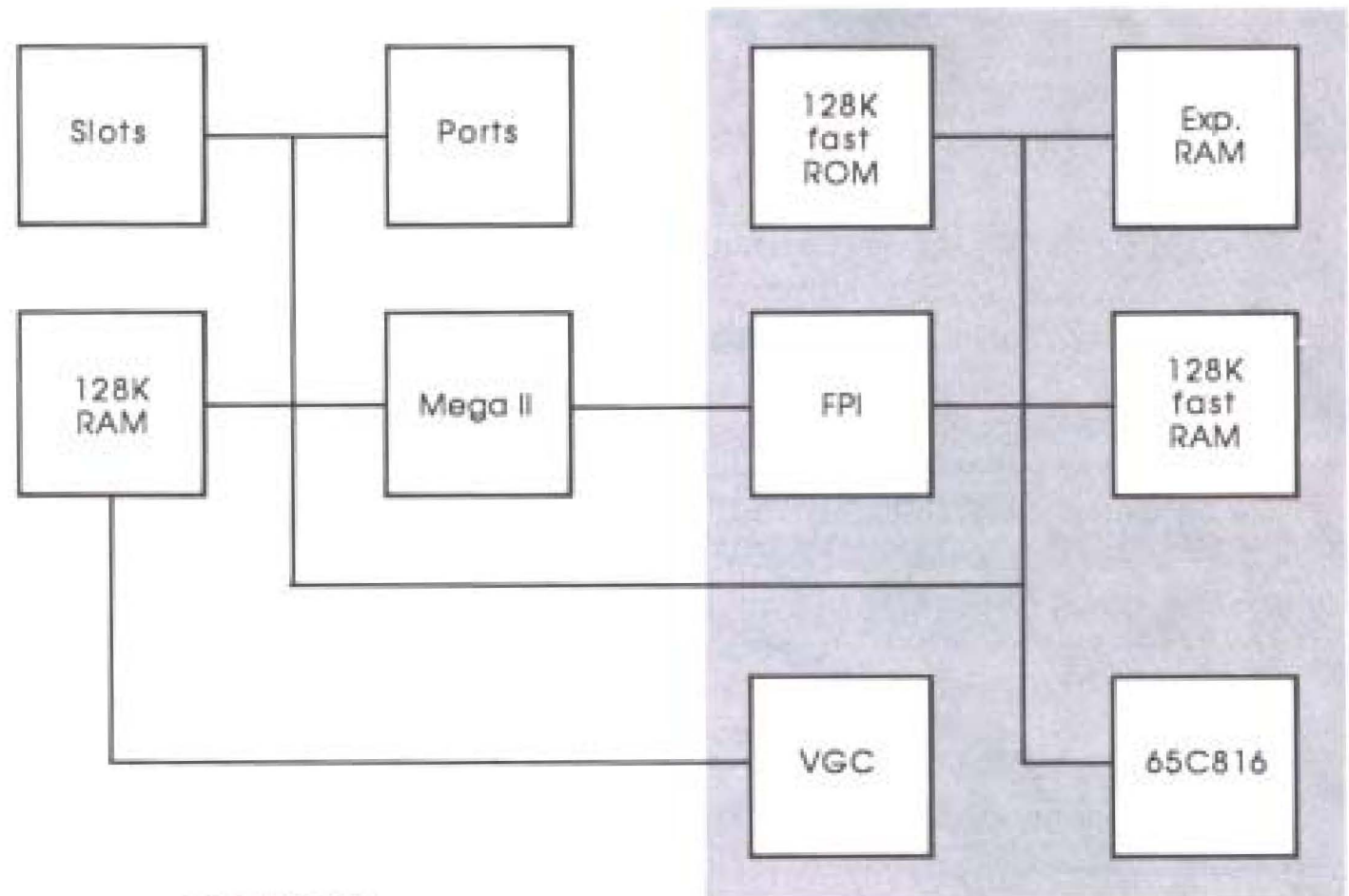
Figure 6-2 New hardware added to the Apple II
