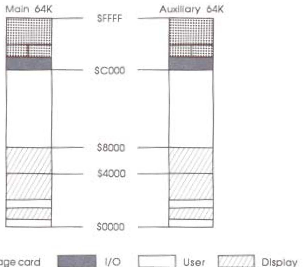
Figure 2-3 128K Apple II memory map
