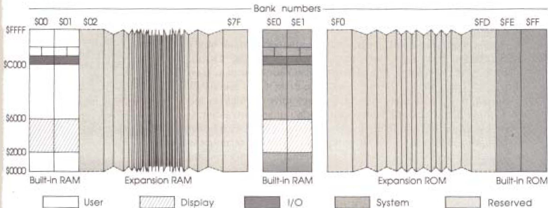
Figure 6-3 Memory map for standard Apple II programs
