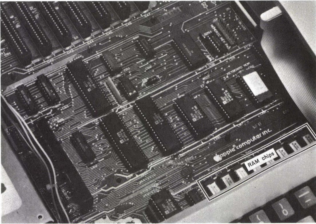
FIG. 5-12 Location of RAM chips on the IIe. Courtesy of Apple Computer, Inc.
