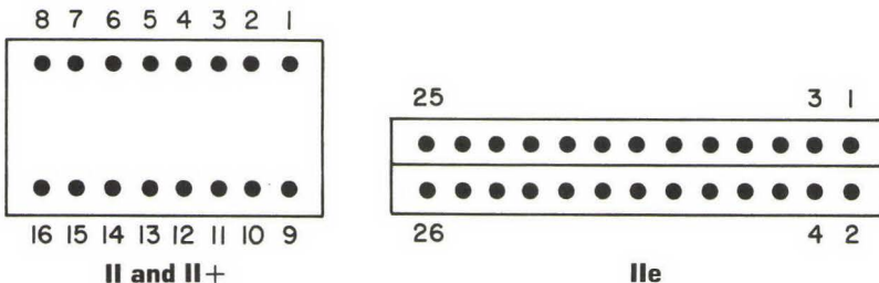
FIG. 6-10 Pin locations on keyboard cable.
