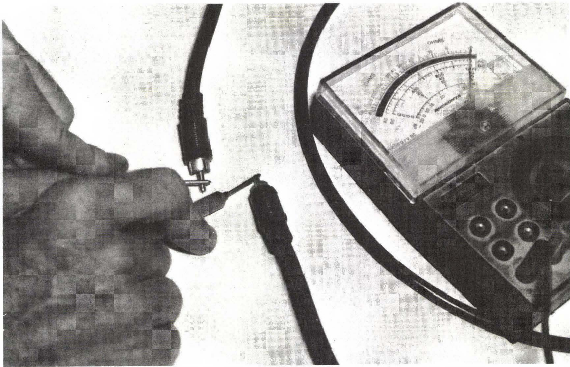
FIG. 6-11 Testing monitor cable for continuity.
