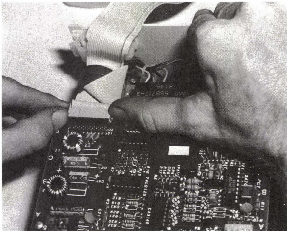
FIG. 4-32 Very carefully remove signal cable from the analog card.
