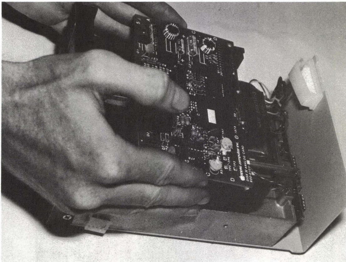
FIG. 4-35 Gently lift analog card free.
