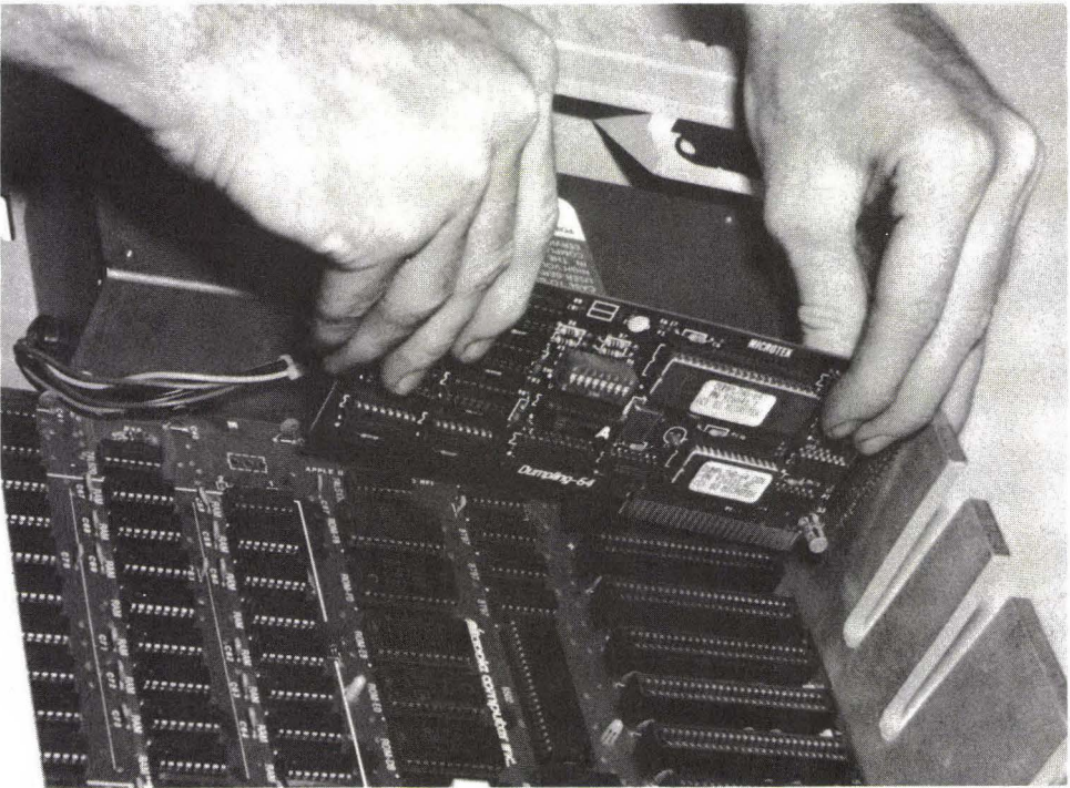
FIG. 6-3 Disconnecting internal devices.
