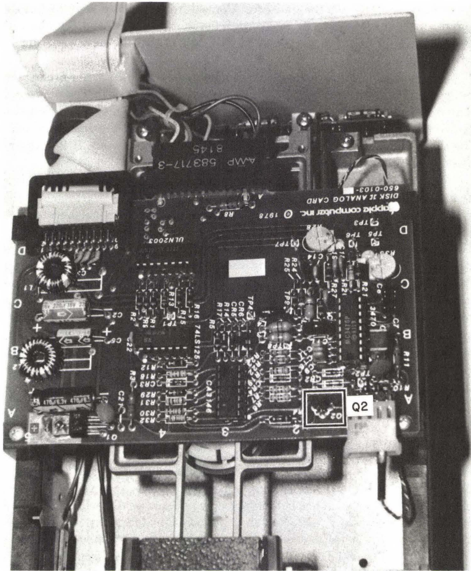
FIG. 4-20 Location of transistor Q2.
