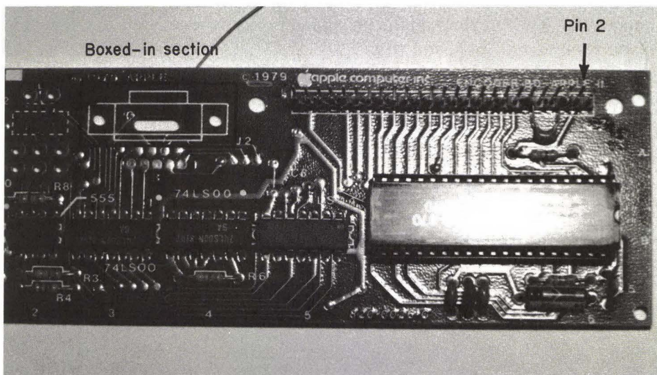
FIG. 8-2 Location of pin 2 and boxed-in section.
