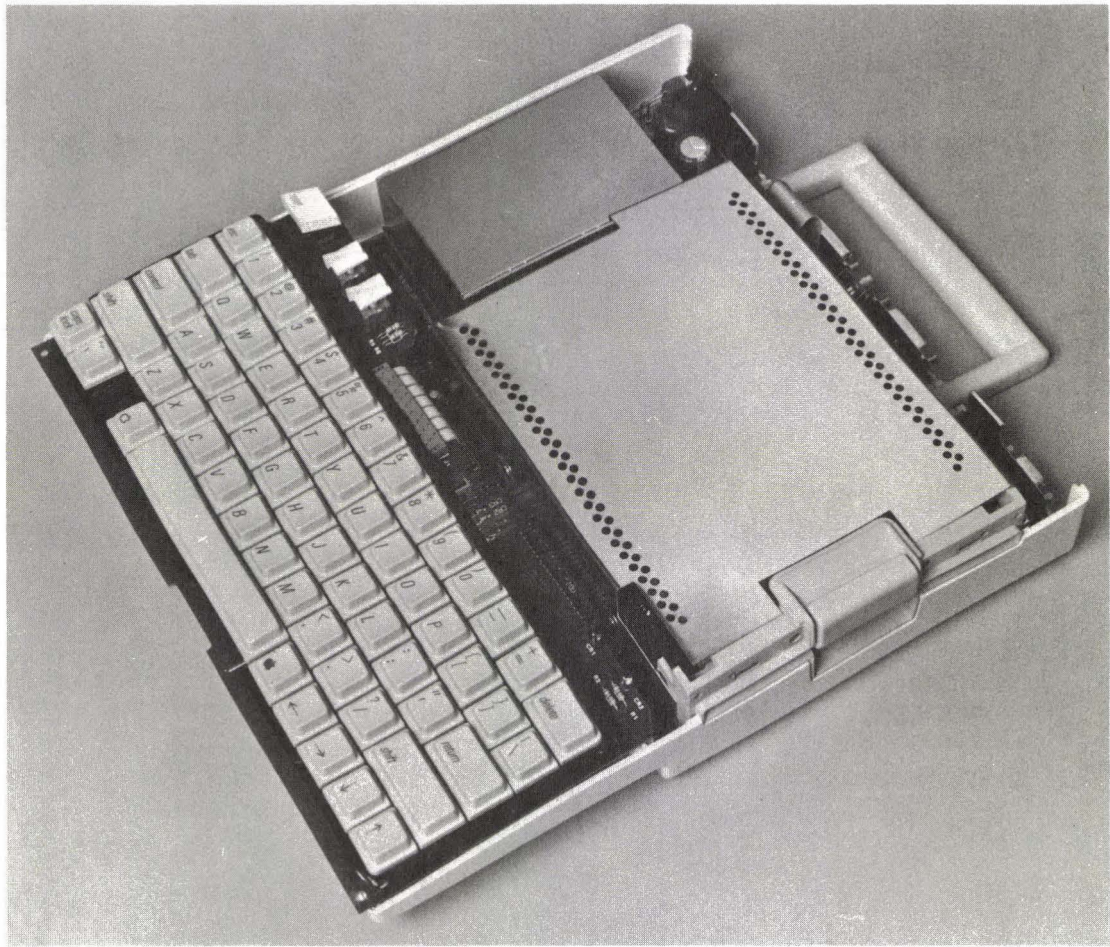
FIG. 10-4 Inside the cabinet. Courtesy of Apple Computer, Inc.
