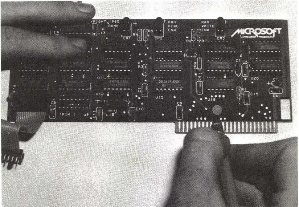
FIG. 6-12 Cleaning the contacts of a board.
