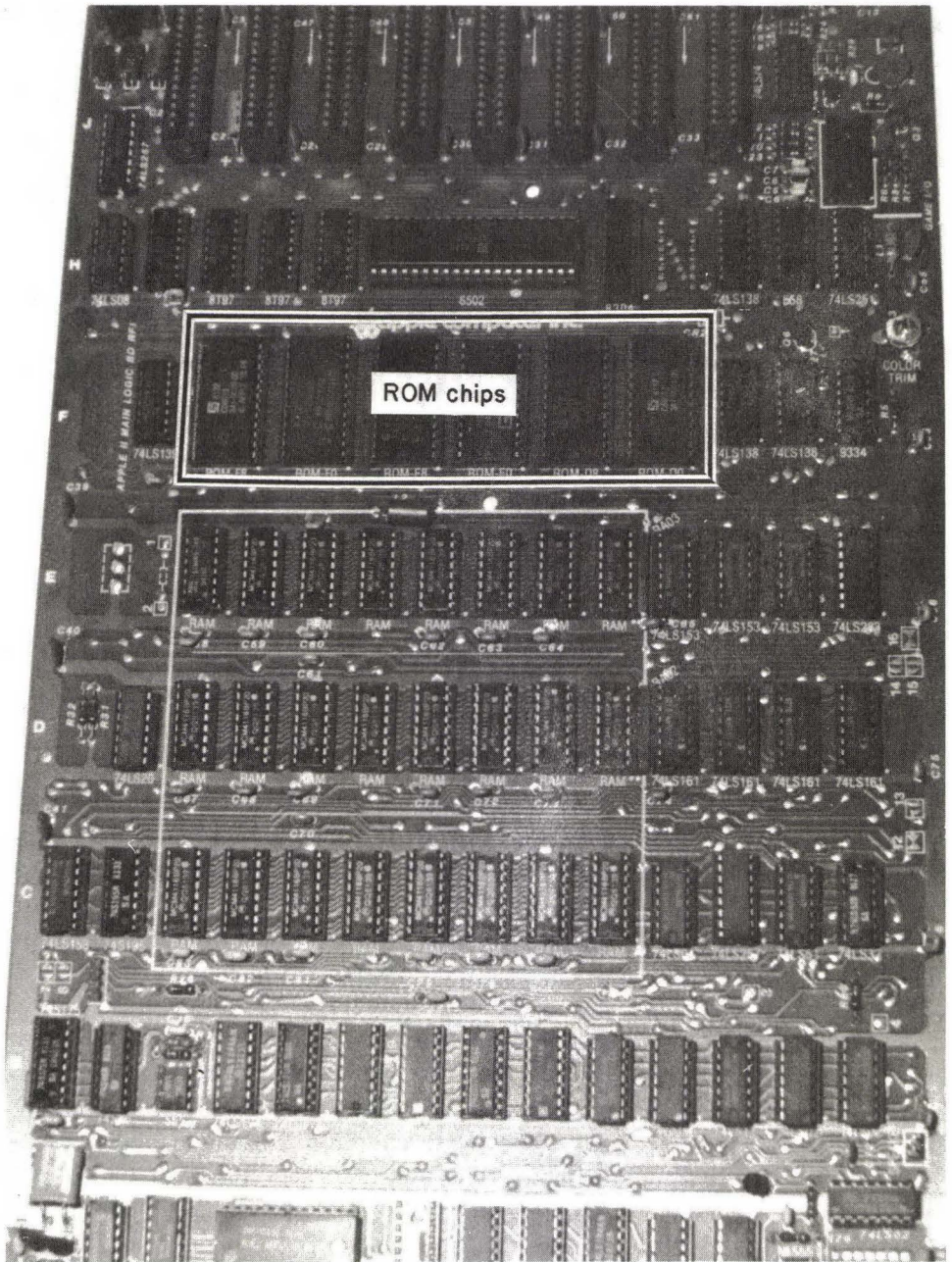
FIG. 5-5 Location of ROM chips on mother board.
