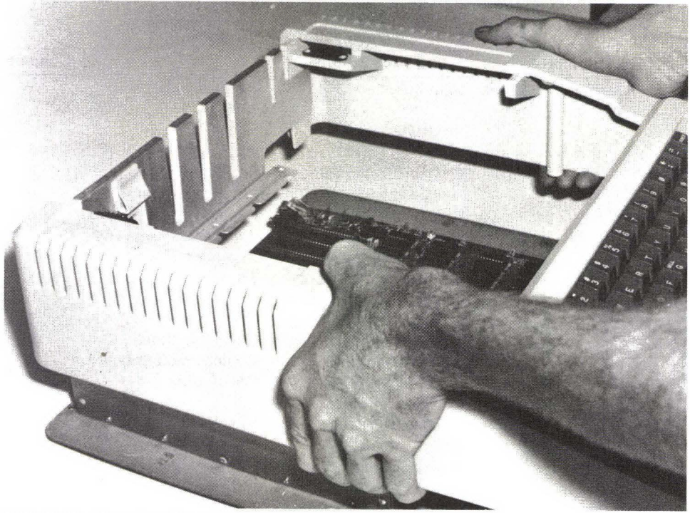
FIG. 2-2 Opening the case.
