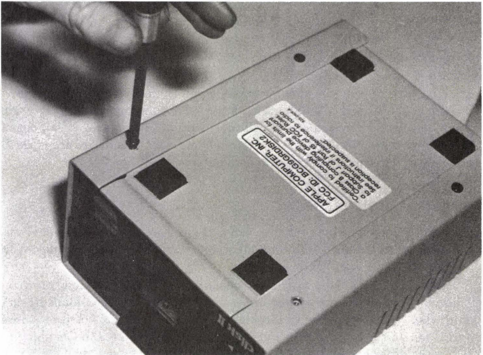
FIG. 4-29 Remove the four holding screws.
