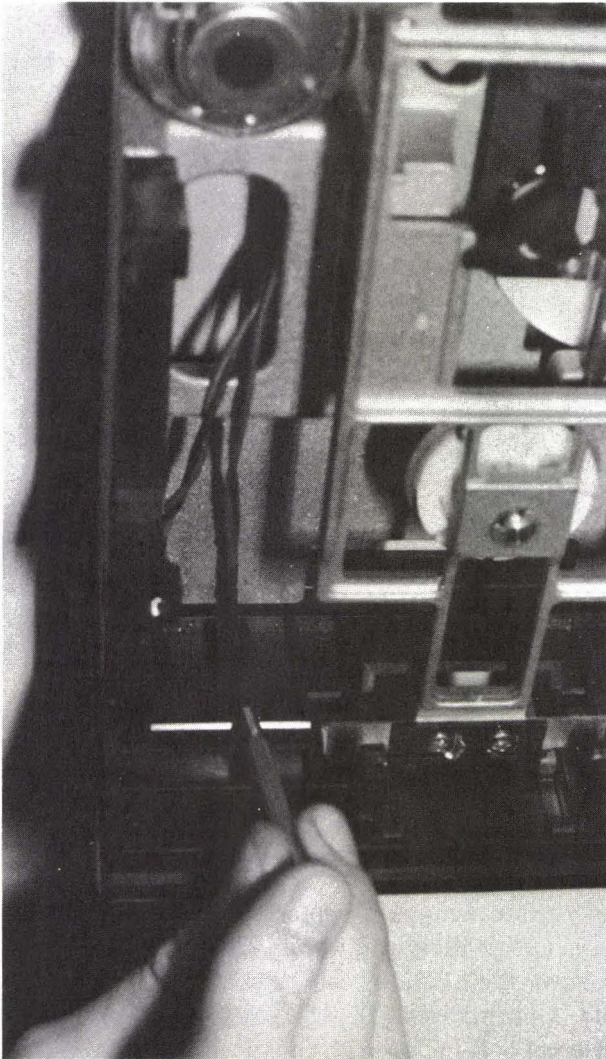
FIG. 4-12 Replacing the drive LED.
