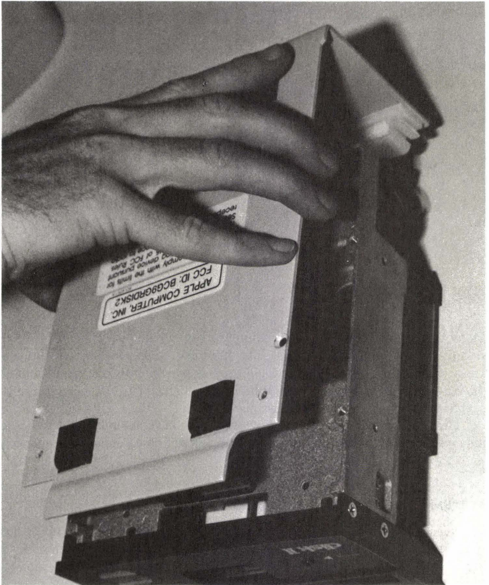
FIG. 4-37 Lift the bottom cabinet off.
