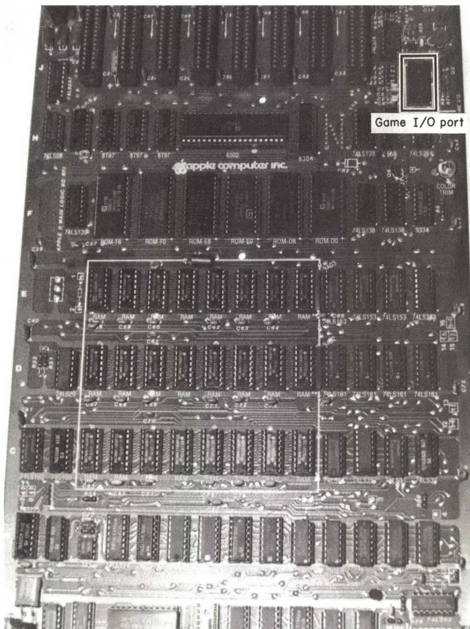
FIG. 5-1 The mother board.
