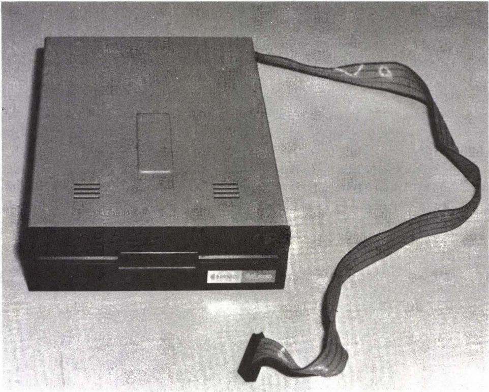
FIG. 4-2 BMC half-height drive.
