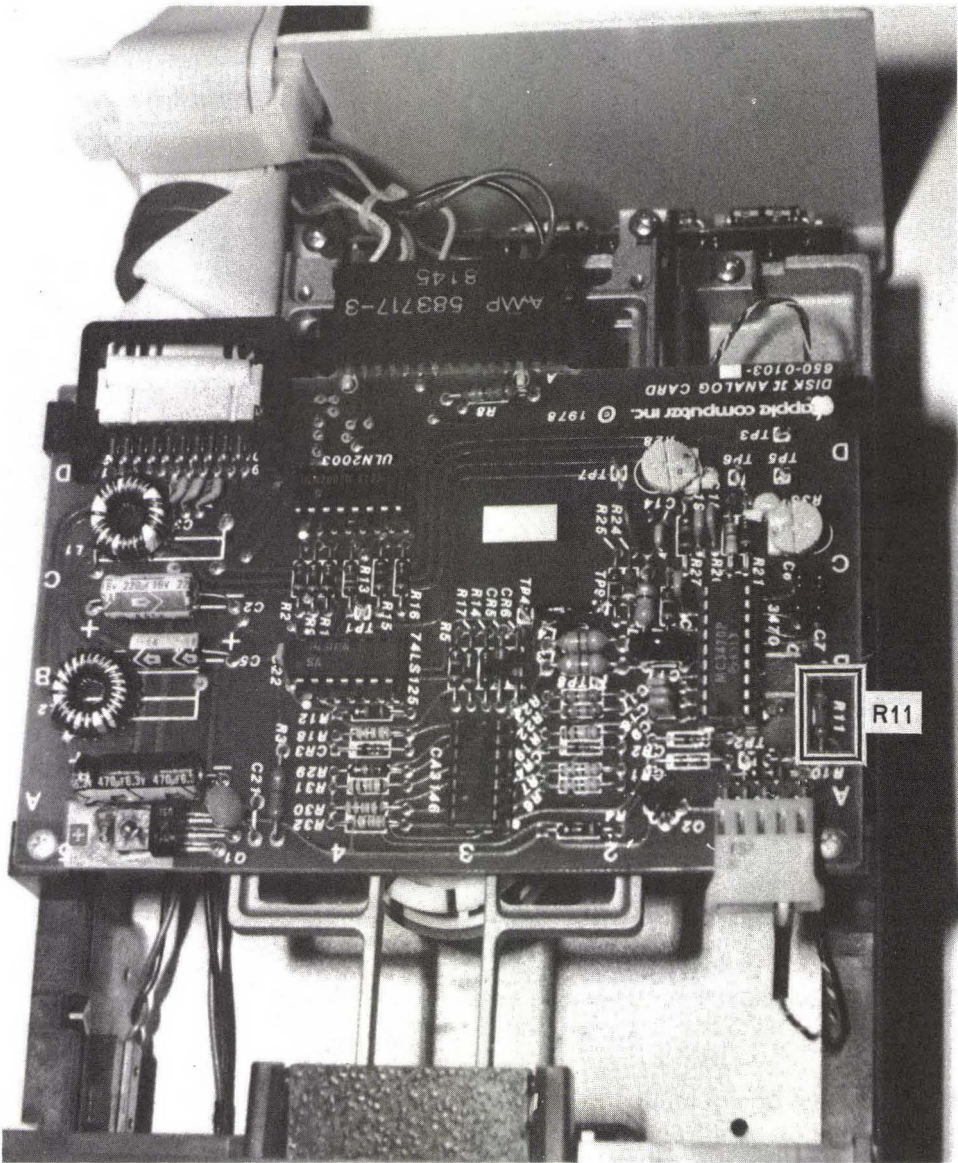
FIG. 4-19 Location of resistor R11.
