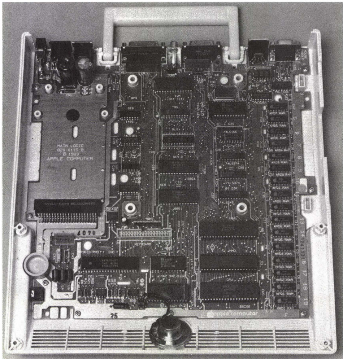
FIG. 10-5 The IIc mother board. Courtesy of Apple Computer, Inc.
