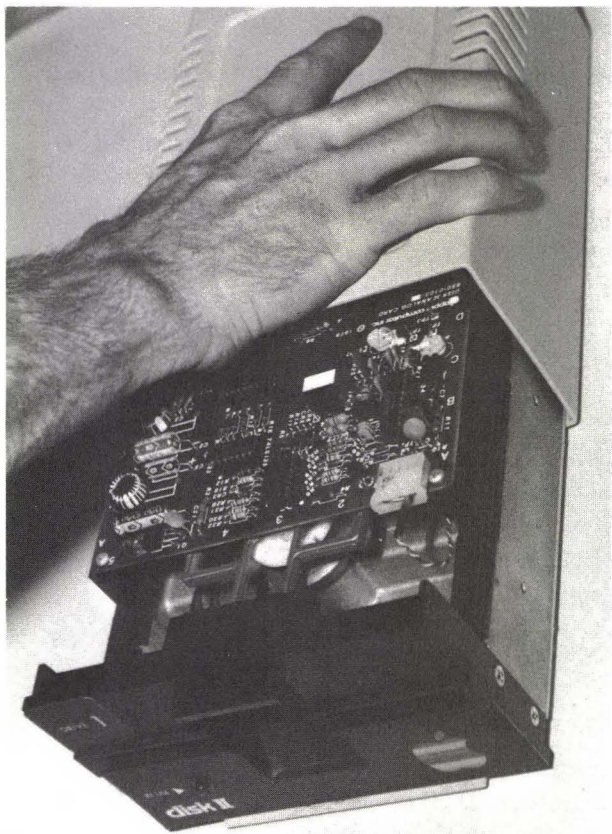
Fig. 4-30 (A) Gently slide the cabinet off (B) The drive with the top cabinet removed.
