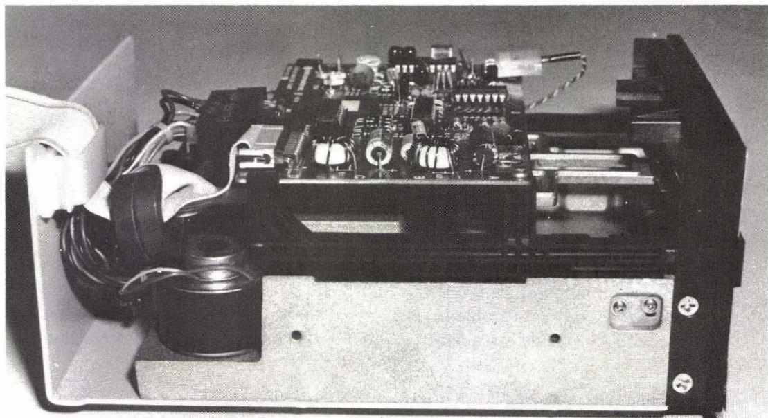
Fig. 4-30 (A) Gently slide the cabinet off (B) The drive with the top cabinet removed.
