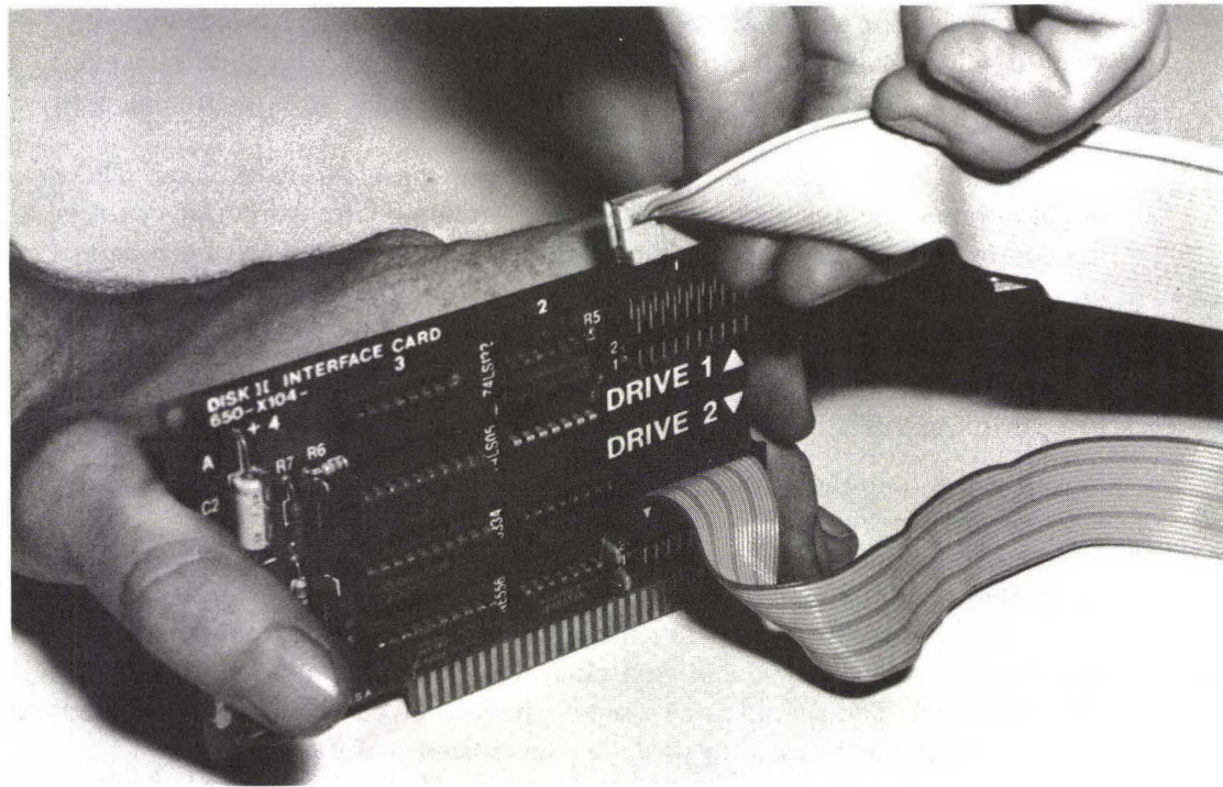
FIG. 4-5 Swapping the drive cables.
