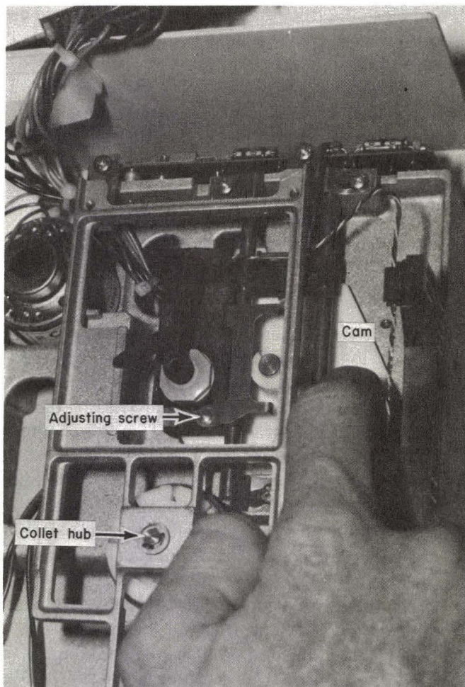
FIG. 4-9 Adjusting screw.
