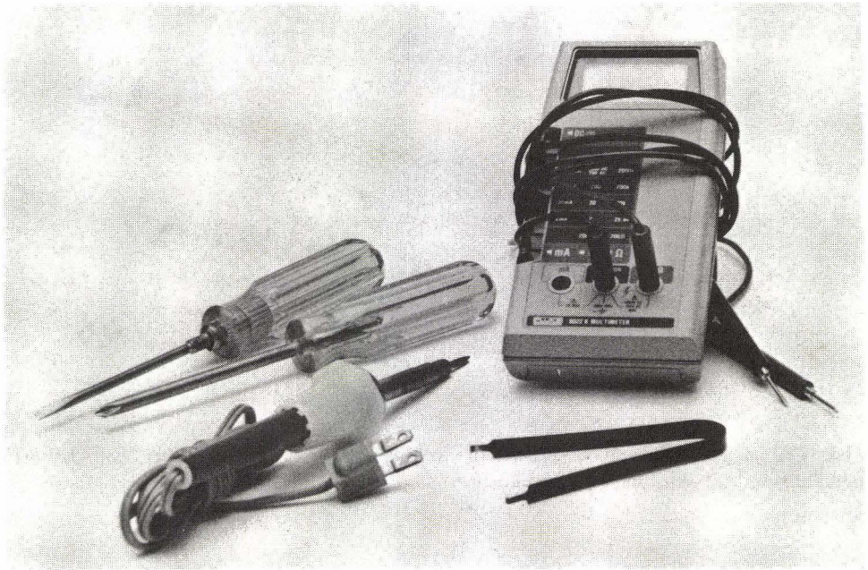
FIG. 1-1 Required tools: screwdrivers, multimeter, soldering tool, and IC extractor.
