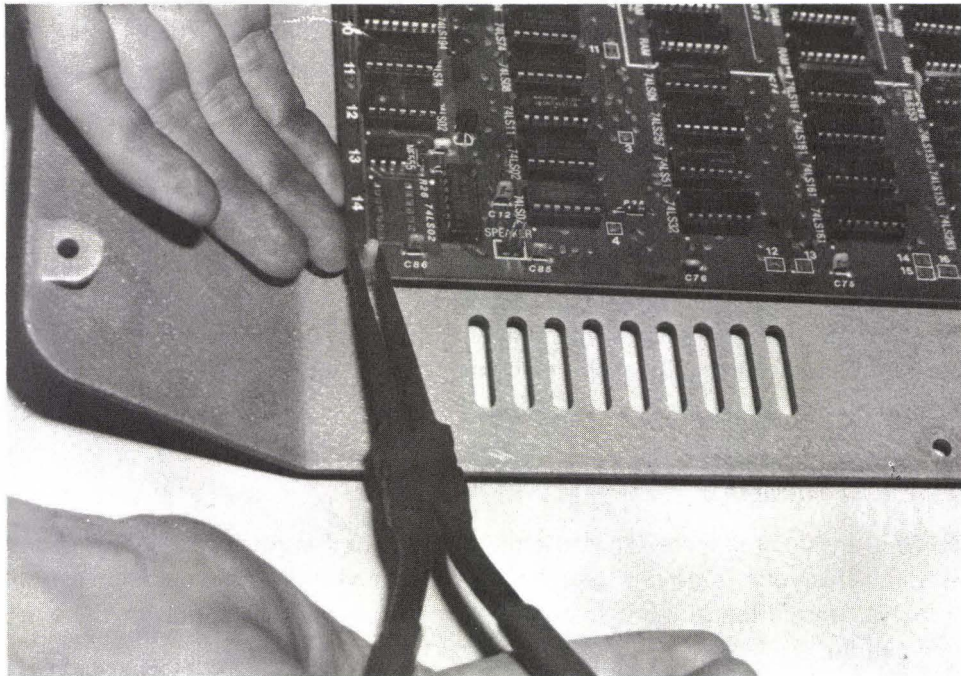
FIG. 5-10 Removing the mother board.
