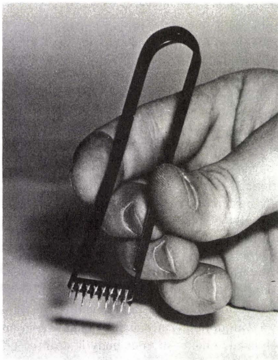
FIG. 1-4 The prongs of an IC are delicate, and the inside can be ruined by static. Handle with care: use an IC extractor for removal.
