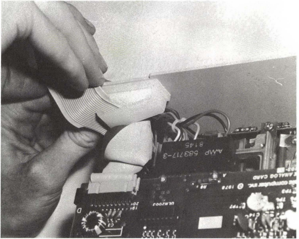
FIG. 4-31 Remove signal cable from clamp.
