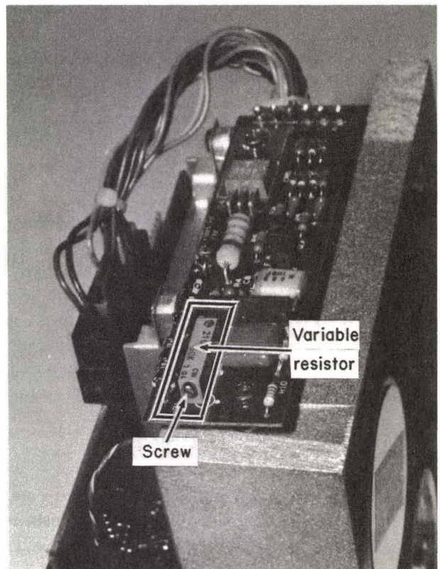
FIG. 4-26 Variable resistor.
