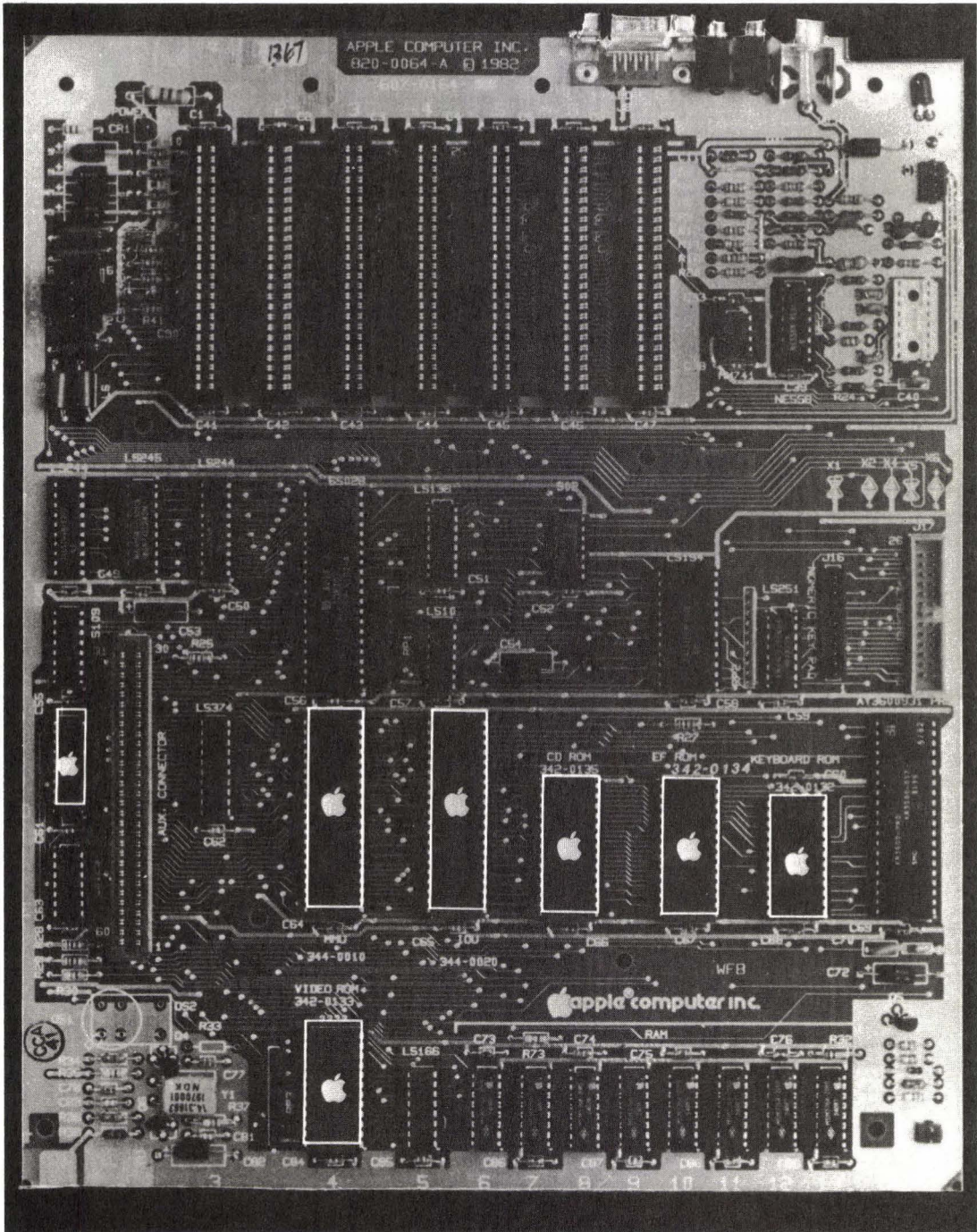
FIG. 5-2 The mother board. Courtesy of Apple Computer, Inc.
