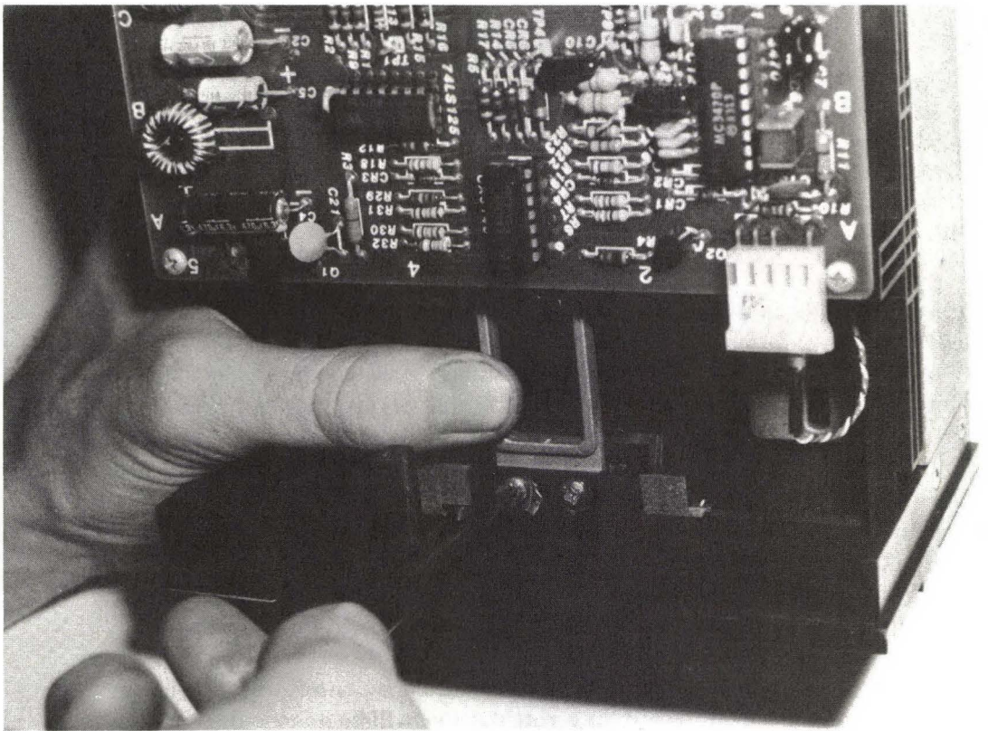
FIG. 4-3 Remove the door assembly screws.
