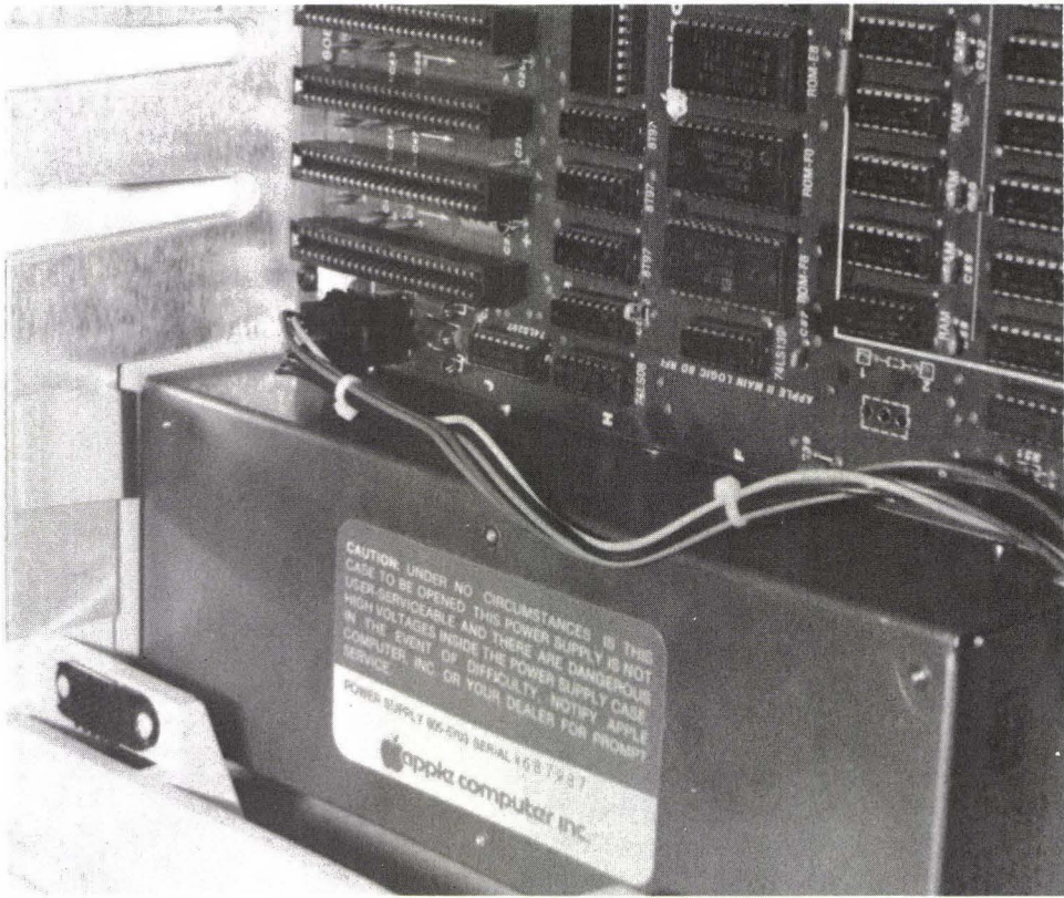
FIG. 5-3 Location of mother board power connector.
