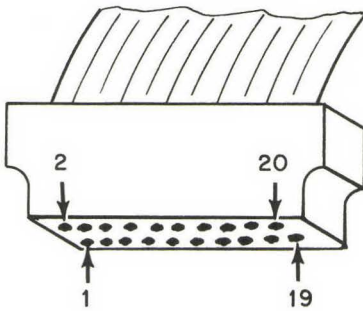
FIG. 4-14 Pin locations on drive signal cable.
