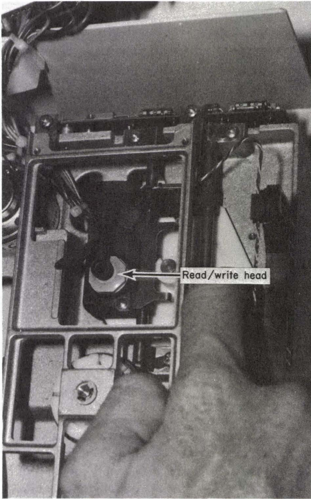
FIG. 4-24 Read/write head.
