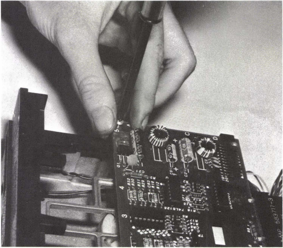
FIG. 4-34 Remove the analog card holding screws.
