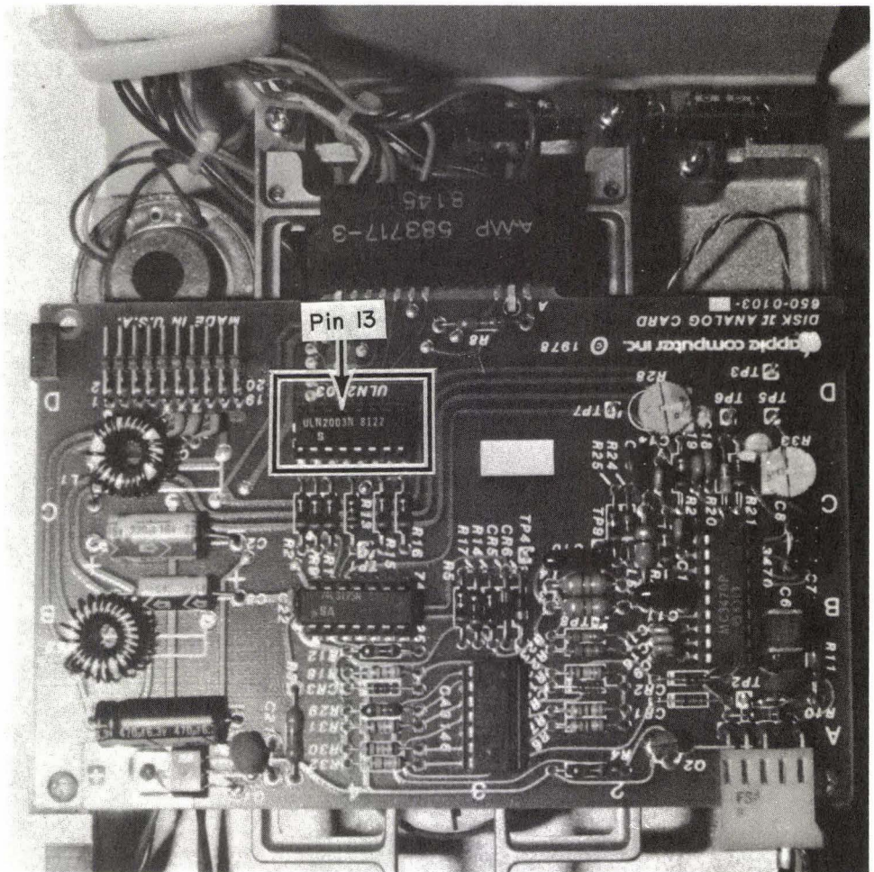
FIG. 4-18 Location of pin 13 on the ULN2003 chip.
