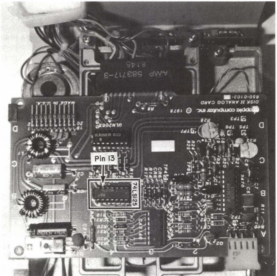
FIG. 4-17 Location of pin 13 on the 74LS125 chip.
