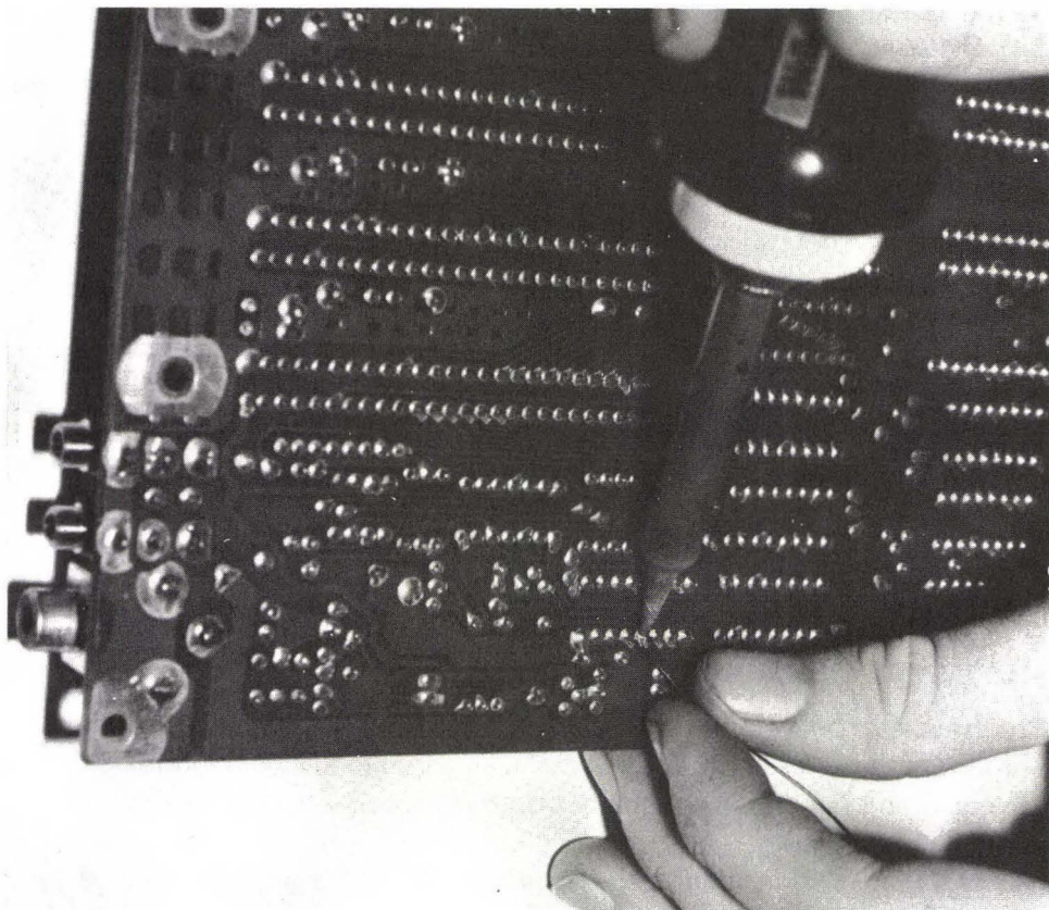
FIG. 8-1 Attaching the wire to pin 4 of the game I/O.
