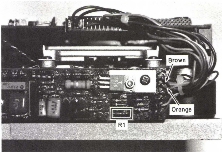
FIG. 4-16 Drive servo board.
