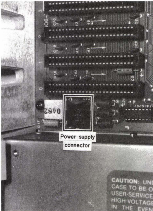
FIG. 6-9 Location of mother board power supply connector.
