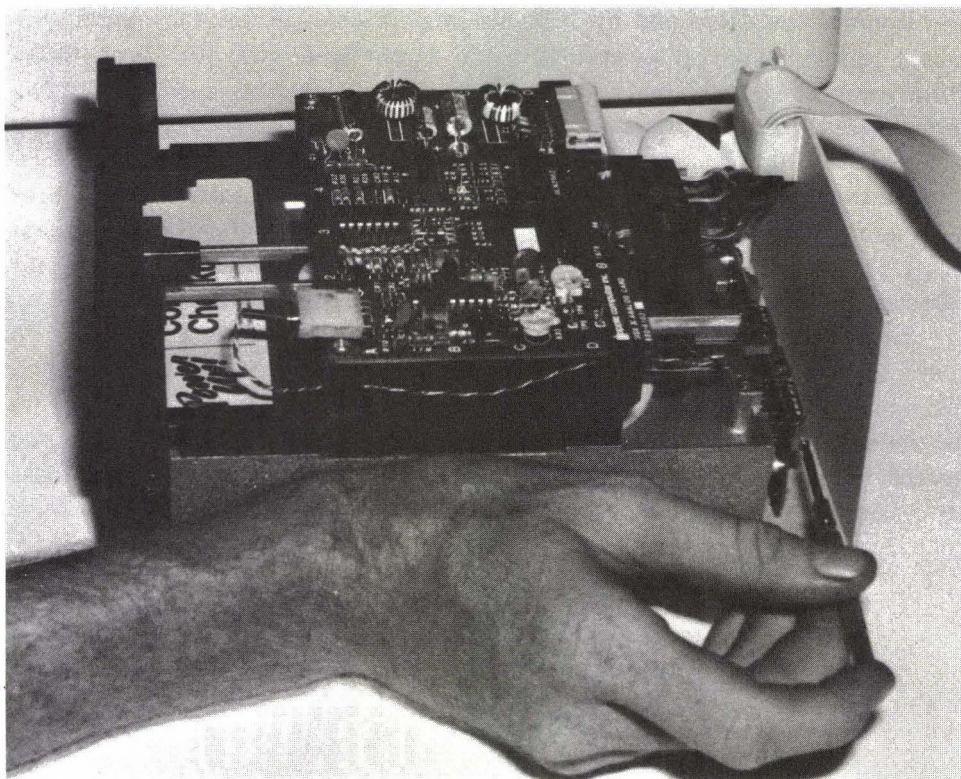
FIG. 4-27 Use a screwdriver to adjust the variable resistor screw.
