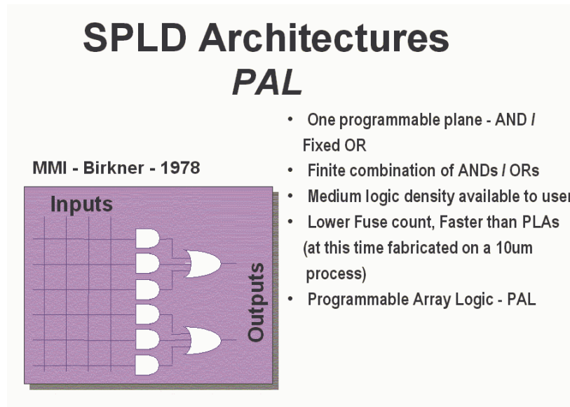
FIGURE 1-2: SPLD ARCHITECTURES
