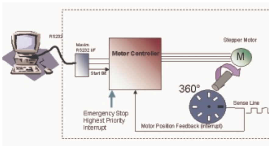
FIGURE 7-5: DESIGN PARTITIONING
