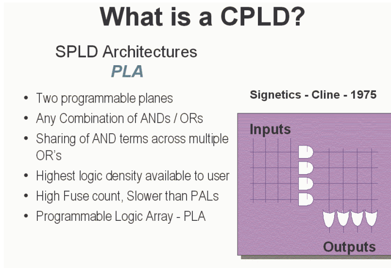
FIGURE 1-1: WHAT IS A CPLD?
