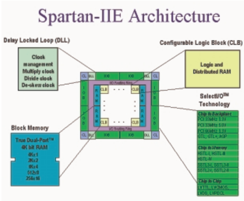
FIGURE 2-8: SPARTAN-IIe ARCHITECTURE
