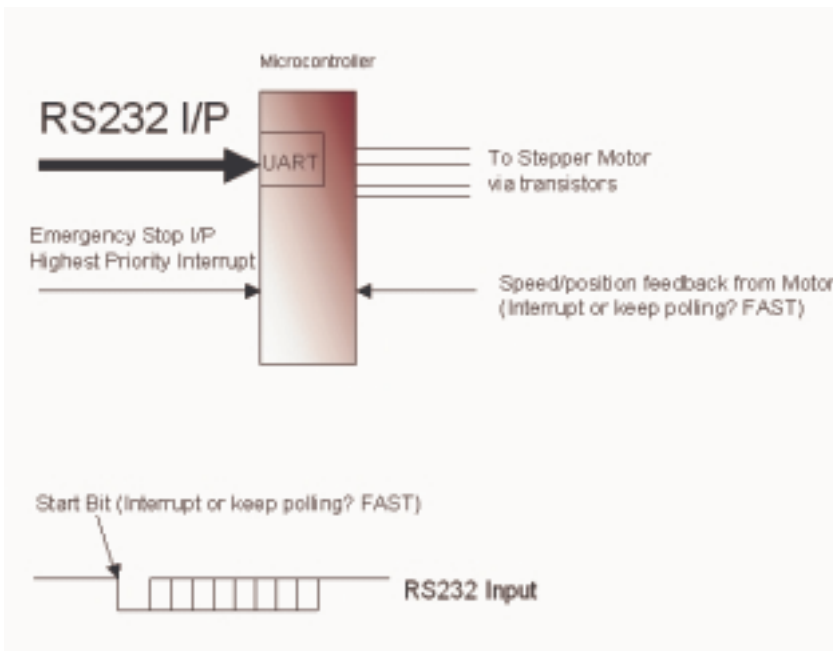
FIGURE 7-6: MICROCONTROLLER IMPLEMENTATION
