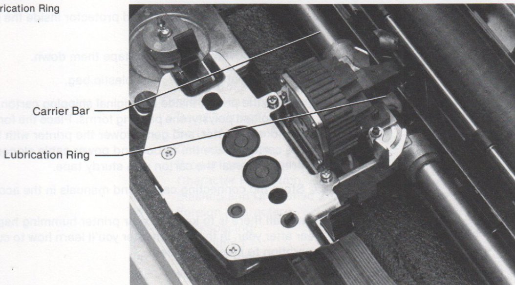
Figure 3-3. Lubrication Ring
