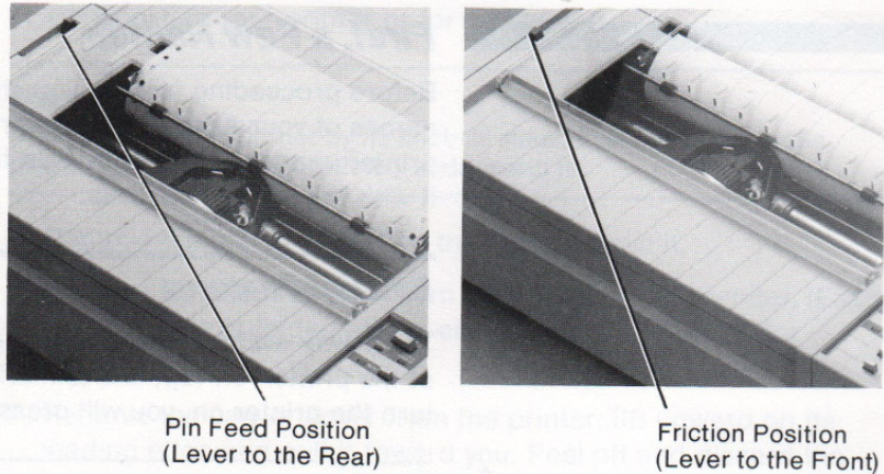
Figure 1-4. Setting the Release Lever
