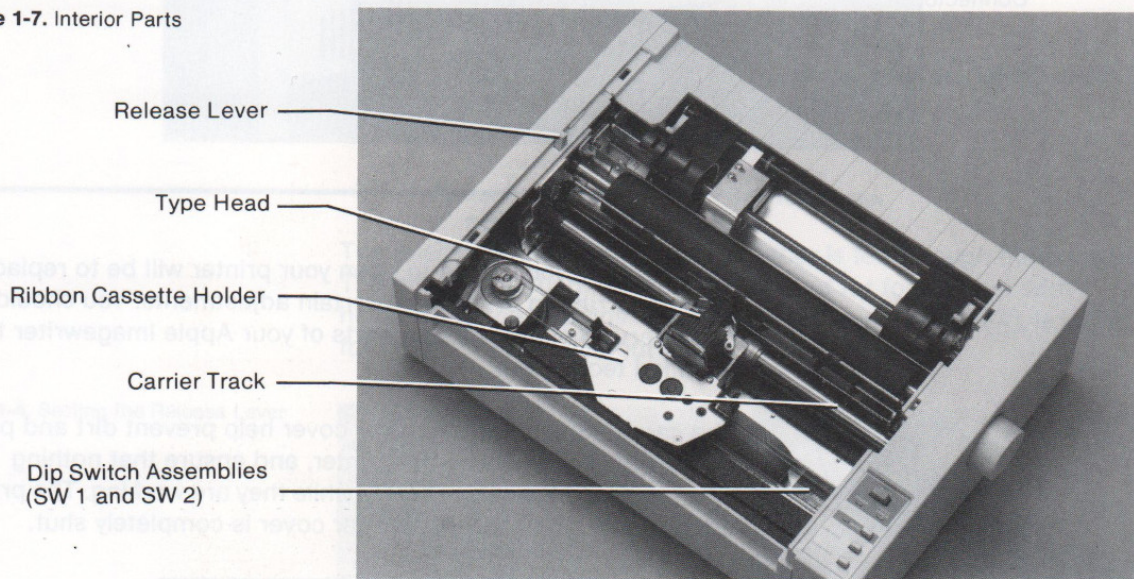
Figure 1-7. Interior Parts
