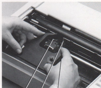
Ribbon Guide Ribbon Guide Plate Cassette Support
