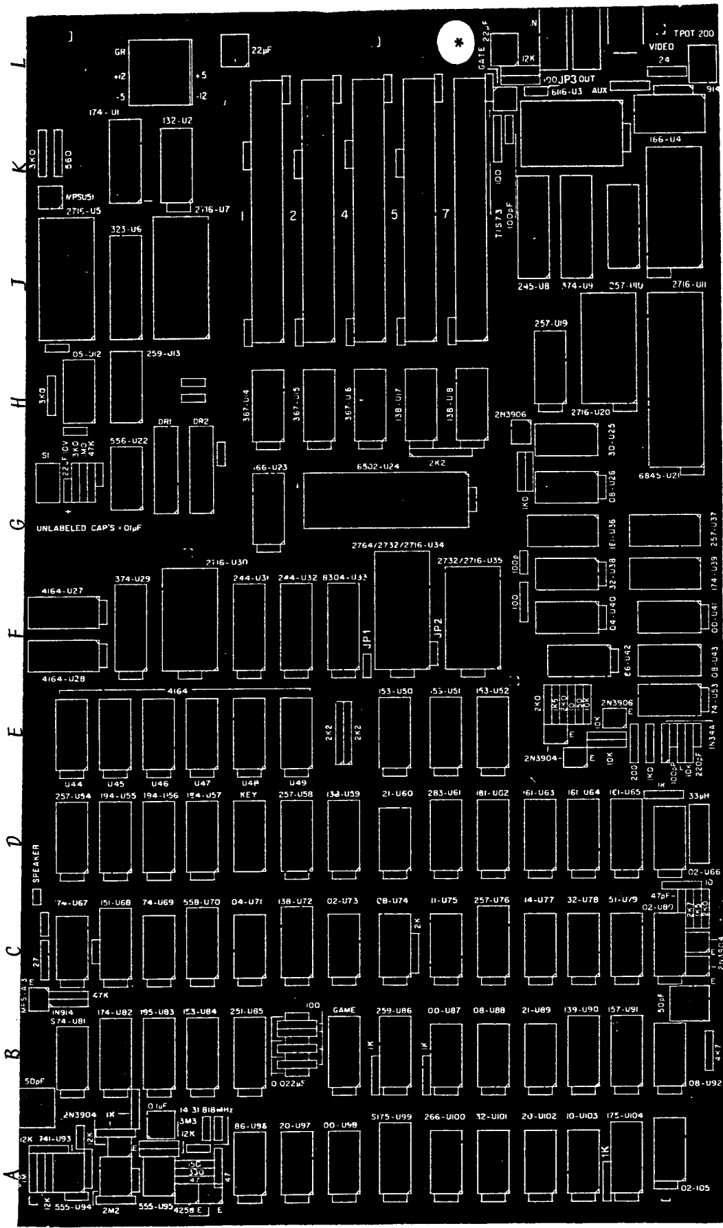
A Fig. 2-16. A COPY OF THE COMPONENT SIDE OF THE SURF-BOARD PCB (REDUCED IN SIZE) SHOWING THE COMPONENT LAYOUT. SOME OF THE UNIQUE FEATURES OF THE SURF-BOARD NOT NORMALLY FOUND ON OTHER SIMILAR PERSONAL COMPUTERS INCLUDE: 64 K BYTES OF USER MEMORY, DUAL DISC DRIVE CONTROLLER; 80-COLUMN TEXT DISPLAY WITH UPPER/LOWER CASE, AS WELL AS HIGH/LOW RESOLUTION COLOUR GRAPHICS, FIVE EXPANSION SLOTS, CASSETTE AND JOYSTICK IN/OUTPUTS, ETC. *The "GATE" of the T1S73 FET transistor is INCORRECTLY silk-screened on the motherboard. Refer to FIG. 5-2, B for correct installation.
