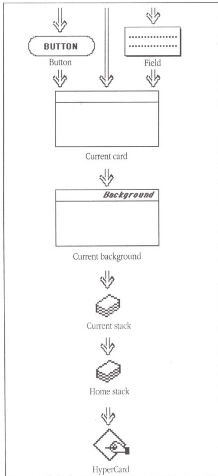
Figure 4-1 The message-passing order
