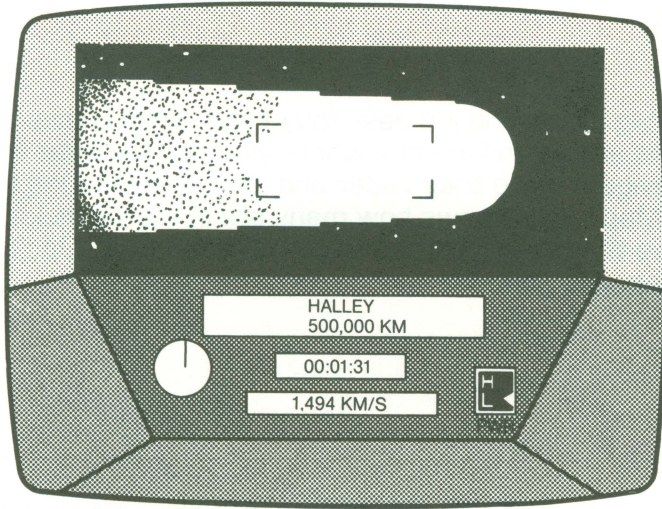
Halley's Comet
