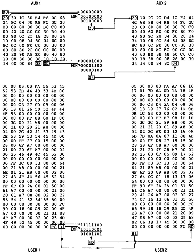
Figure C.12 Example: The Exclusive ORing Operation
