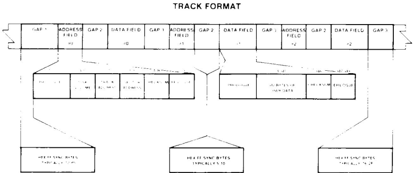
Figure 3.6 Track Format
