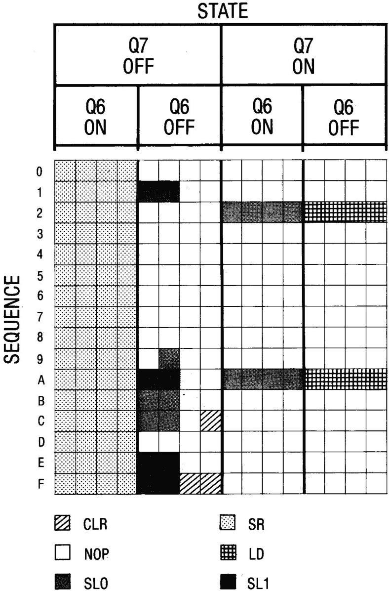
Figure D.2 Sequencer Commands
