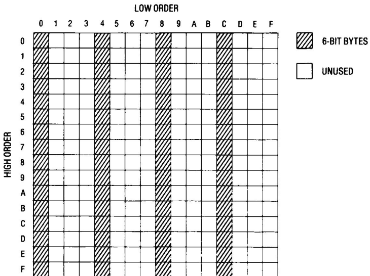
Figure C.3 Valid 6-Bit Bytes
