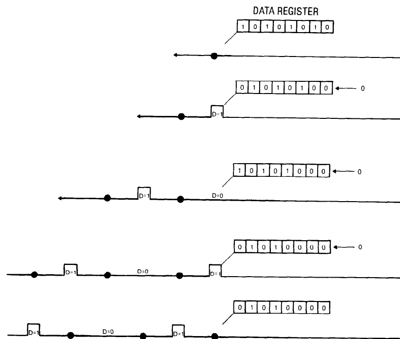
Figure 3.5 Writing Data to a Diskette
