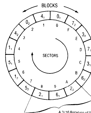
Figure 3.14 Block Interleaving (Track 0)
