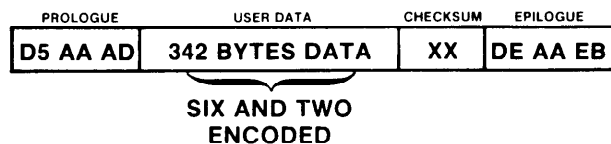
Figure 3.13 Data Field
