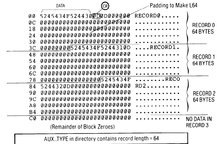
Figure 4.12 Example Random Text File Block
