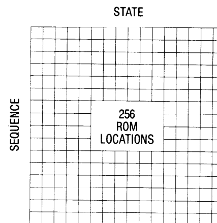
Figure D.1 Sequencer ROM is Addressed by a 4-Bit Input (STATE) and a 4-Bit Control Statement (SEQUENCE)
