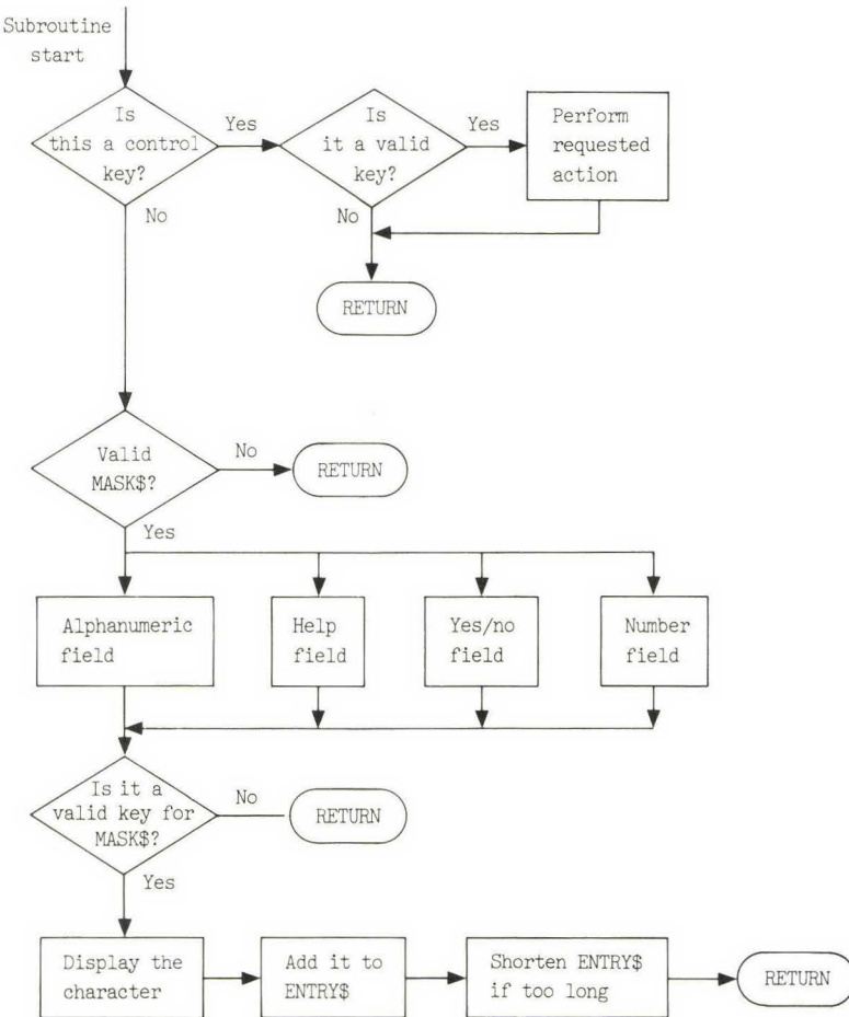
FIG. 2.6 Flowchart for accepting a character
