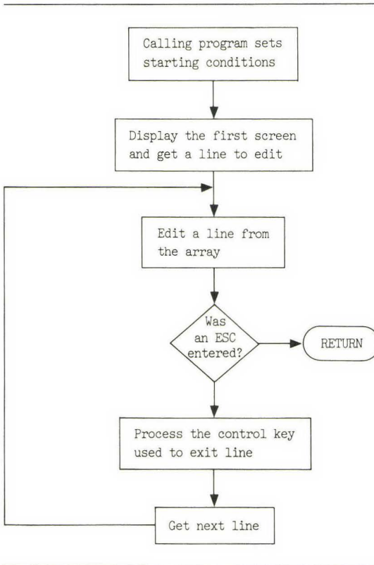
FIG. 3.1 Text editor flowchart
