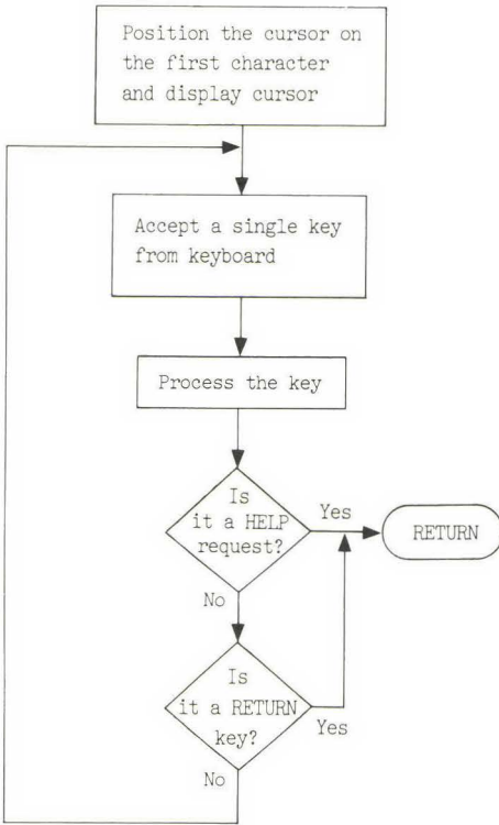
FIG. 2.4 Subroutine for editing the field
