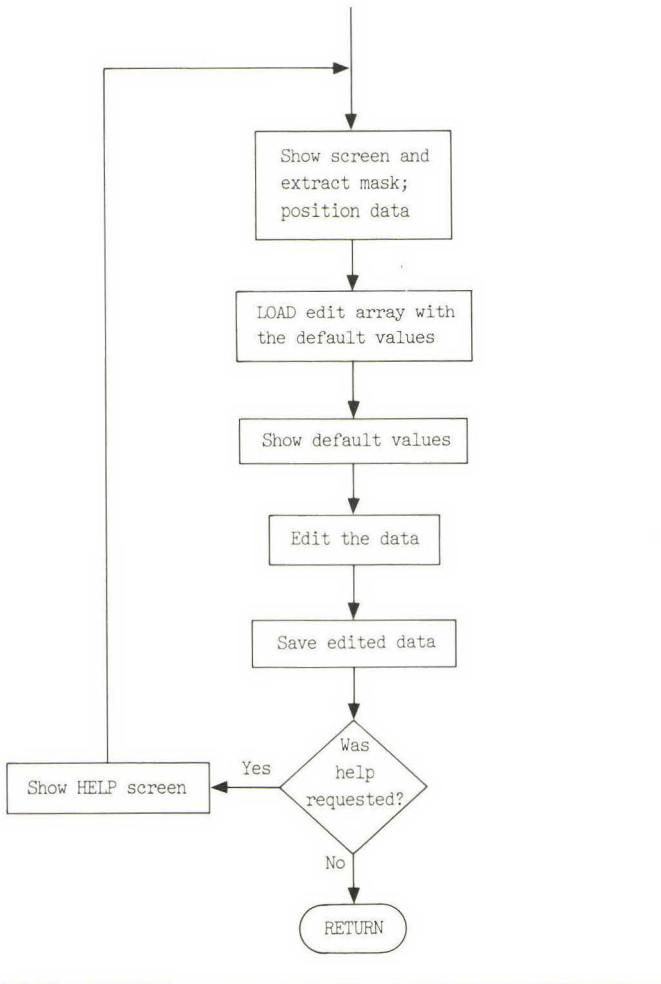
FIG. 5.2 Flowchart for data entry screen processor
