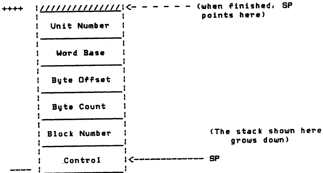
Figure 3.0 -- Stack state on entering UNITREAD or UNITWRITE
