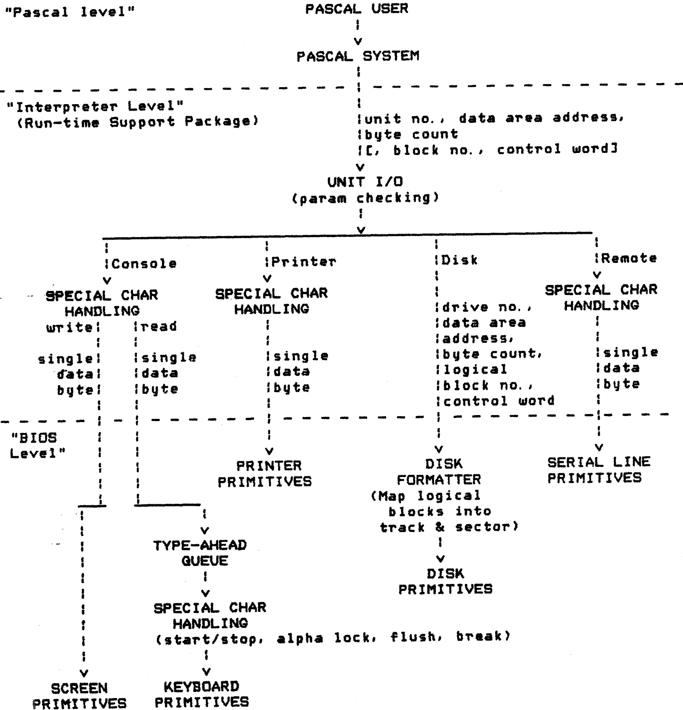
Figure 1.0 -- Pascal I/O System Hierarchy
