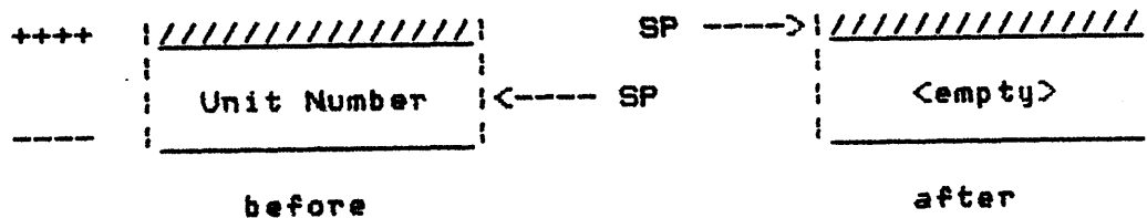
Figure 3.2 -- Stack state before and after UNITWAIT
