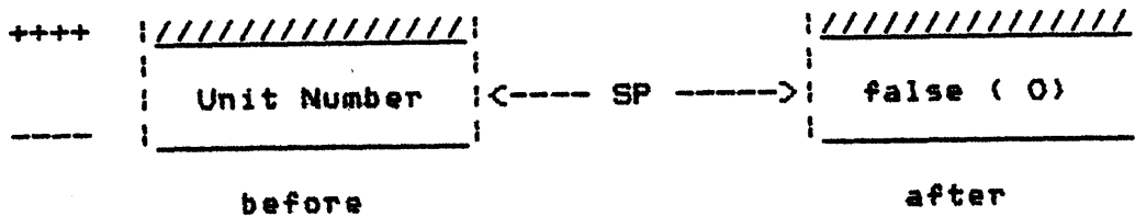
Figure 3.1 -- Stack state before and after UNITBUSY
