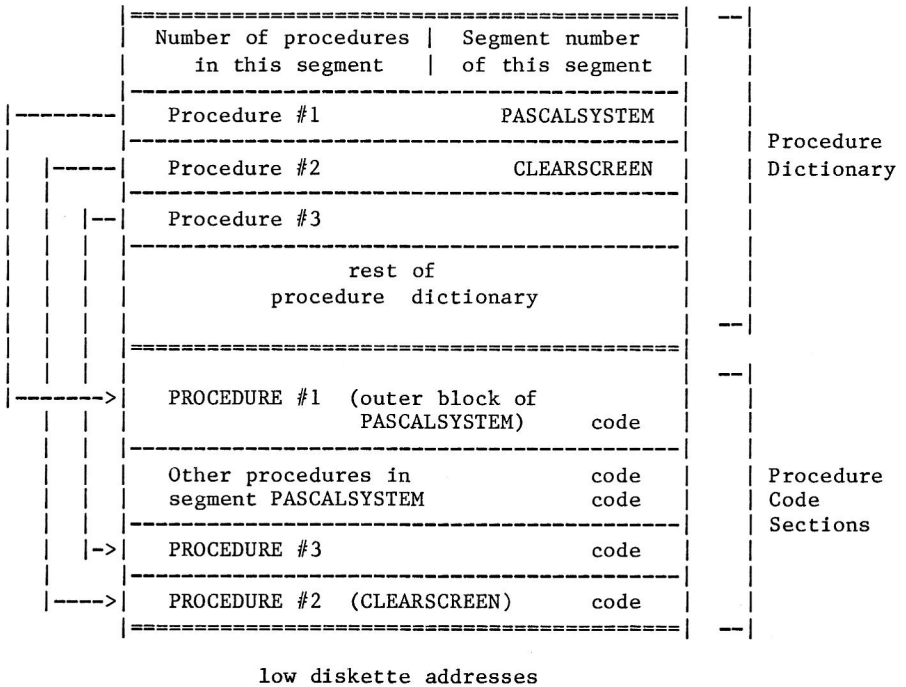
FIGURE 2 DETAIL OF THE "PASCALSYSTEM" CODE SEGMENT
