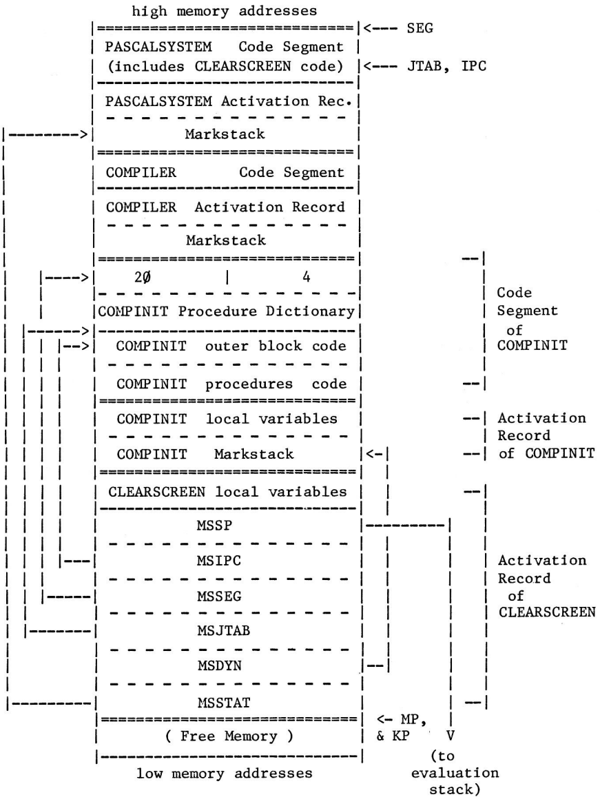
FIGURE 7 DETAIL OF THE PROGRAM STACK DURING EXECUTION OF PROCEDURE CLEARSCREEN
