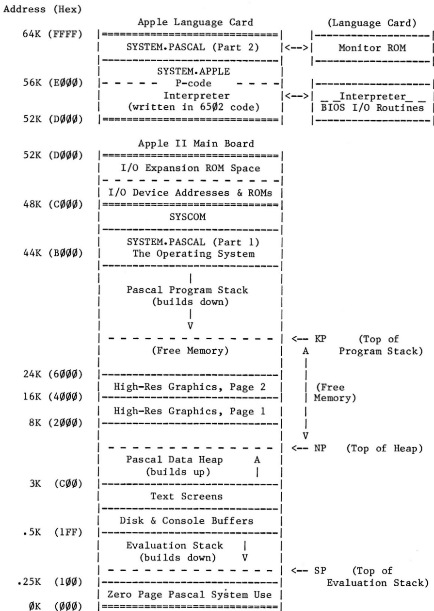
FIGURE 4 MEMORY MAP OF THE APPLE II WHEN USING APPLE PASCAL
