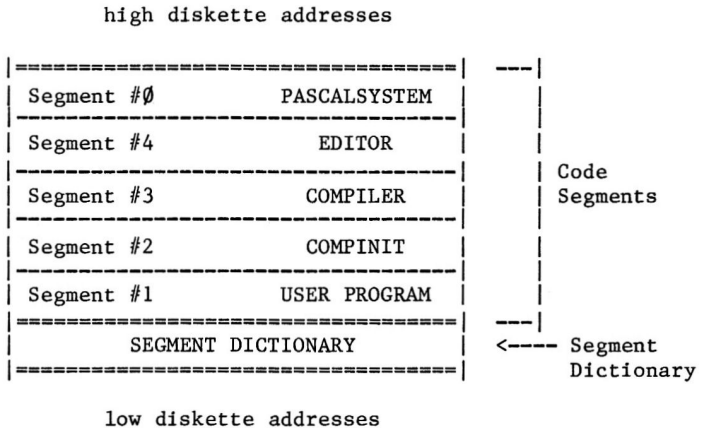
FIGURE 1 COMPLETE CODEFILE OF "THE PROGRAM"
