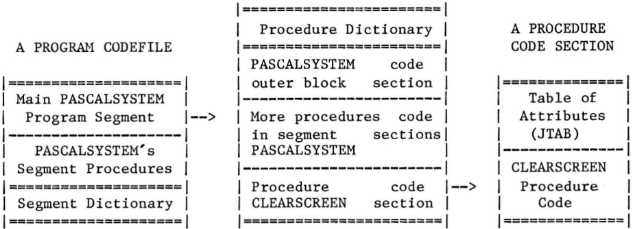
Figure 1 Complete Codefile of "The Program"
