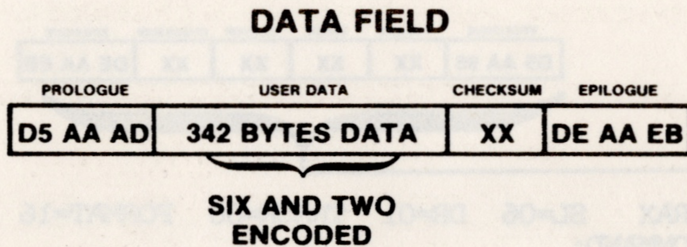
FIGURE 2.3 — DATA FIELD
