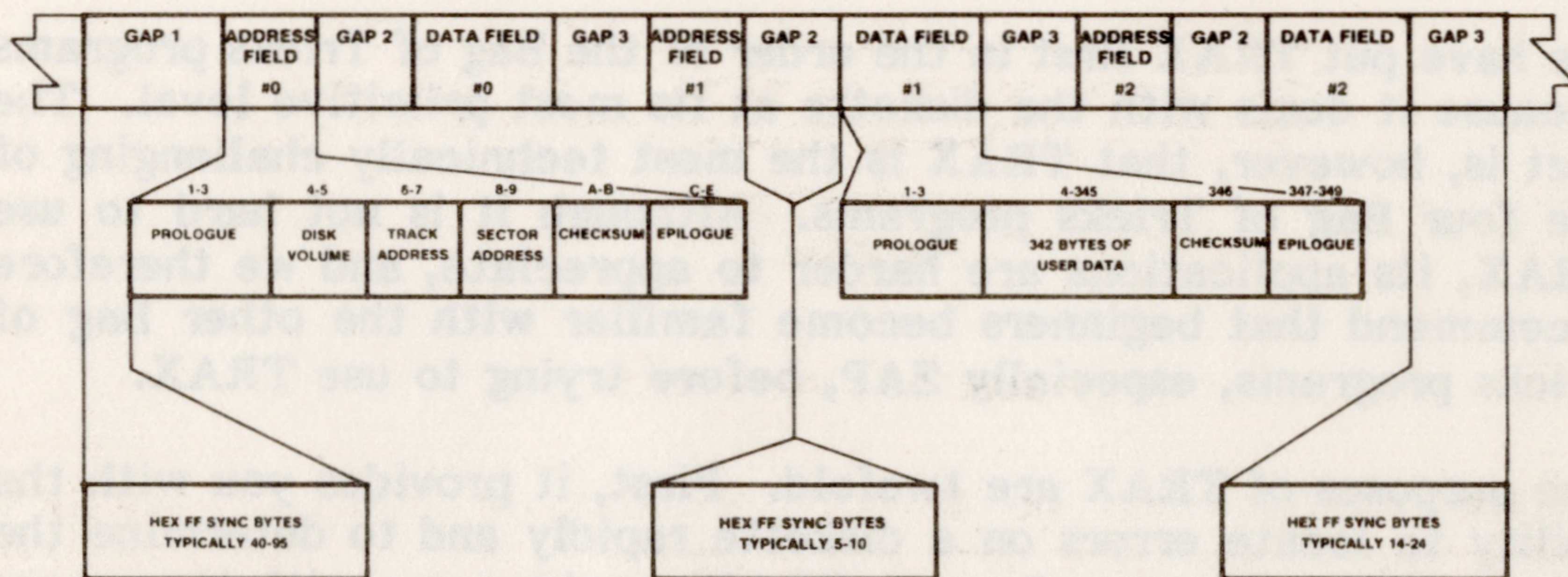
FIGURE 2.1 — TRACK FORMAT
