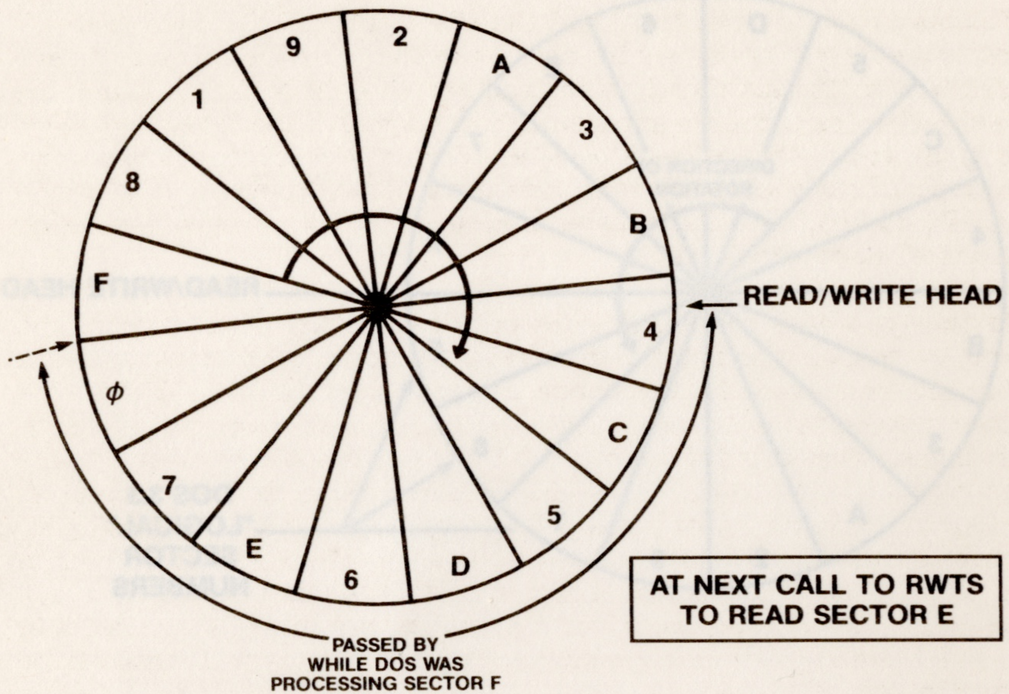
FIGURE 3.5 — STANDARD DISKETTE POSITION AFTER PROCESSING SECTOR F
