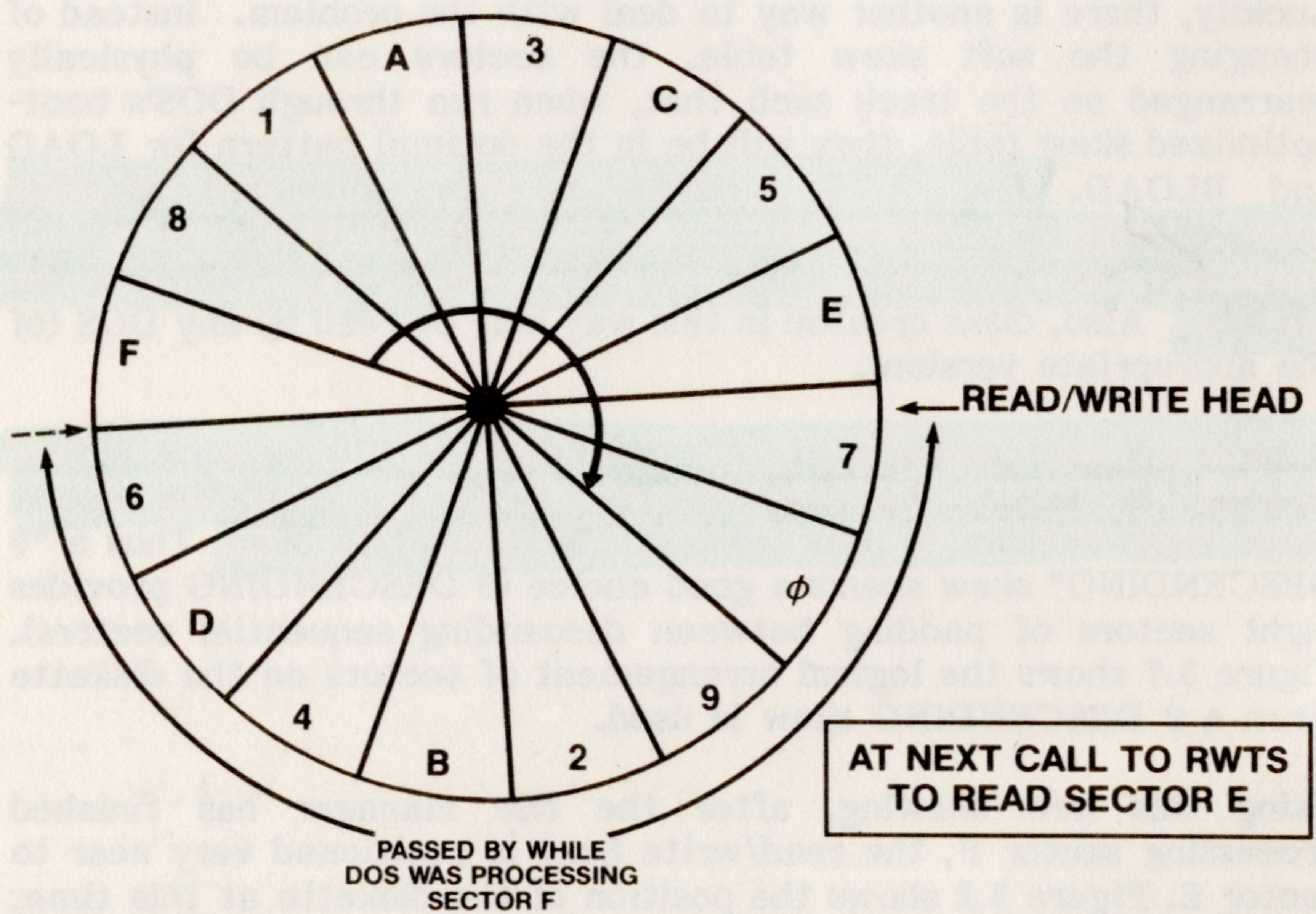
FIGURE 3.8 — 9 DESCENDING SKEW AFTER PROCESSING SECTOR F
