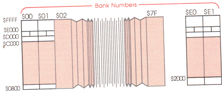
Figure 3-4 Memory allocatable through the Memory Manager
