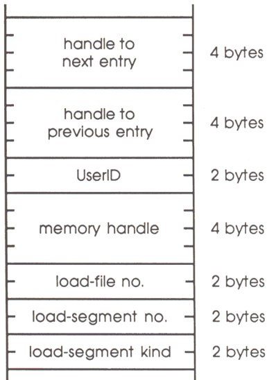
Figure 15-1 Memory Segment Table entry
