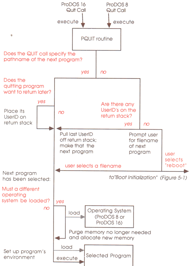
Figure 5-3 Run-time program selection (QUIT call)
