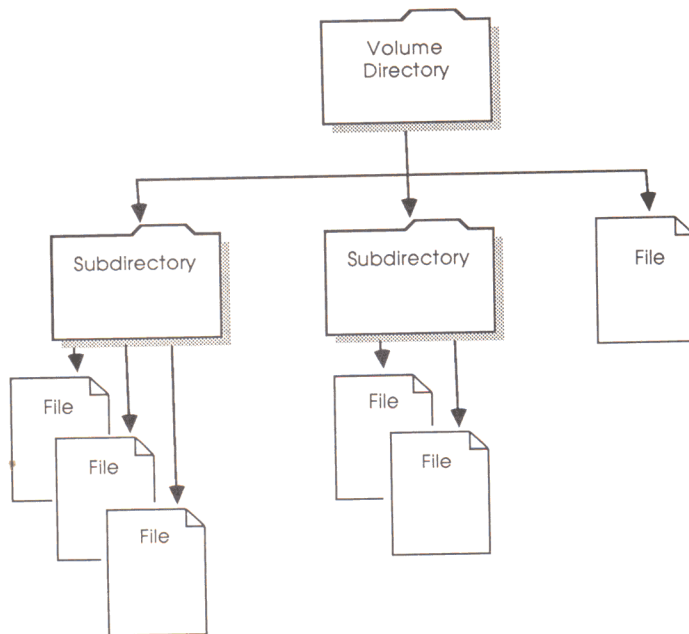
Figure 1-2 Example of a hierarchical file structure
