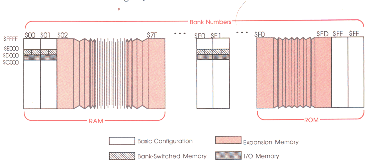
Figure 3-1 Apple IIGS memory map
