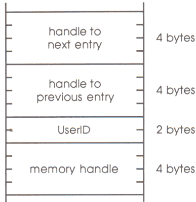
Figure 15-2 Jump Table Directory entry
