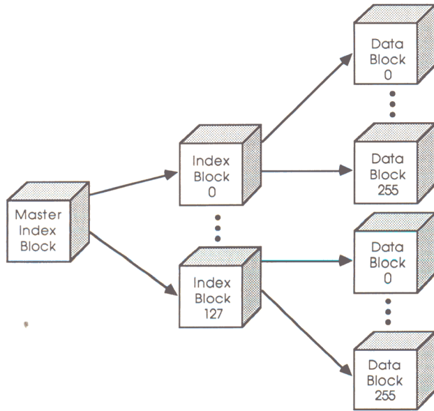
Figure 2-5 Block organization of a standard file
