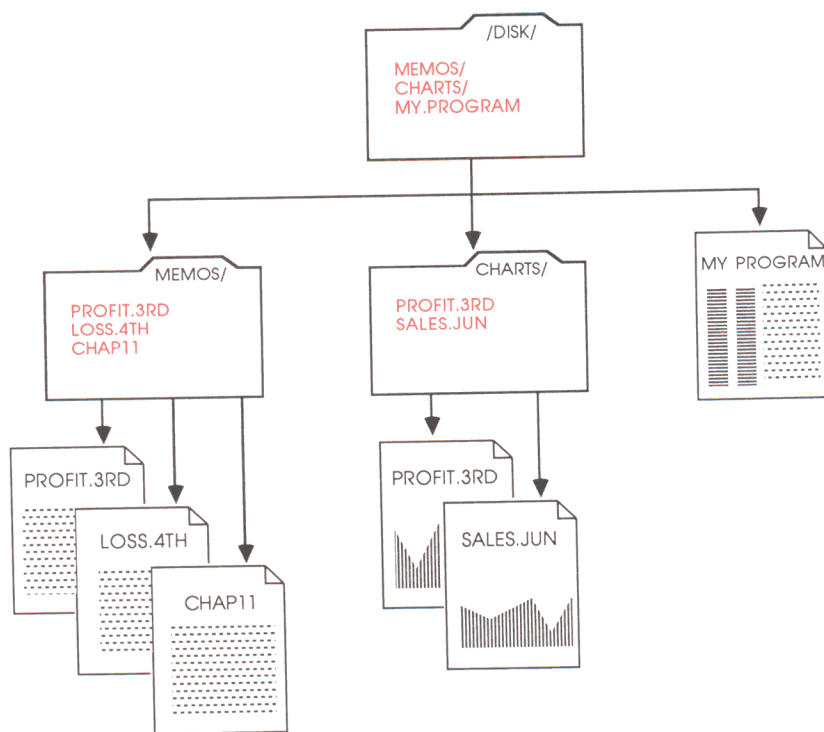
Figure 2-1 Example of a ProDOS 16 file structure
