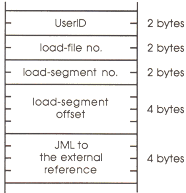
Figure 15-4 Jump Table entry (loaded state)
