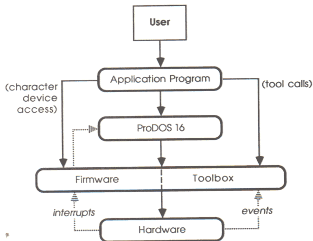
Figure 1-1 Programming levels in the Apple IIGS
