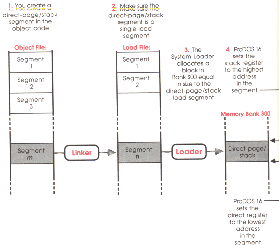
Figure 6-1 Automatic direct-page/stack allocation
