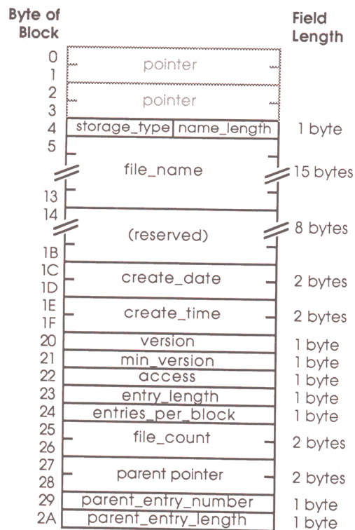
Figure A-4 The subdirectory header
