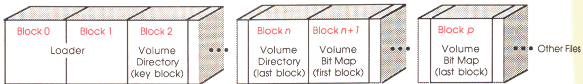
Figure A-1 Block organization of a volume
