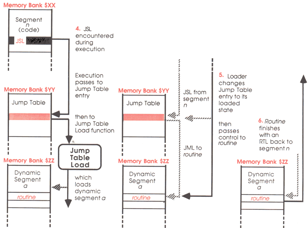
Figure 15-5B How the Jump Table works (continued)
