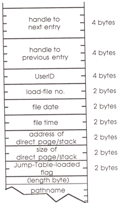
Figure 15-6 Pathname Table entry
