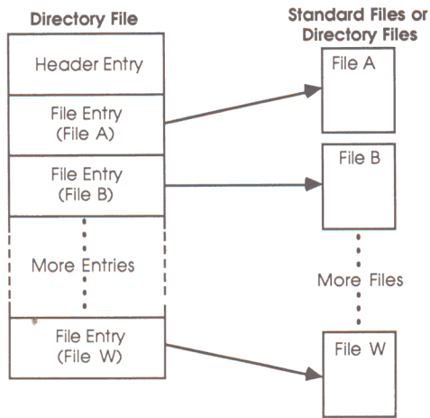
Figure 2-3 Directory file format
