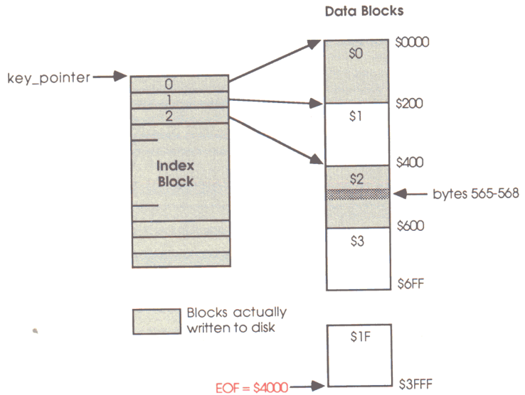
Figure A-9 An example of sparse file organization
