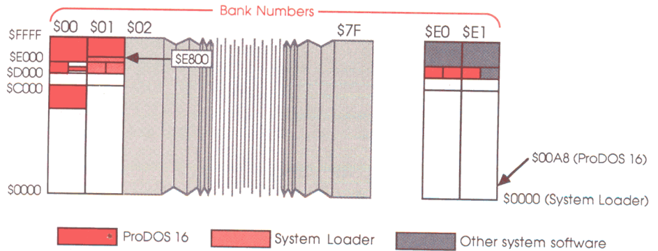
Figure 3-2 ProDOS 16 and System Loader memory map
