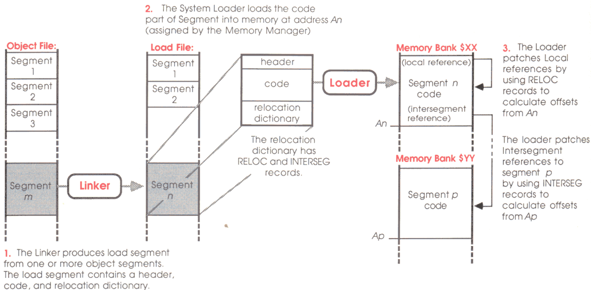
Figure 14-1 Loading a relocatable segment
