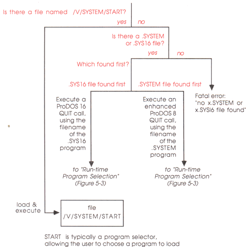
Figure 5-2 Startup program selection
