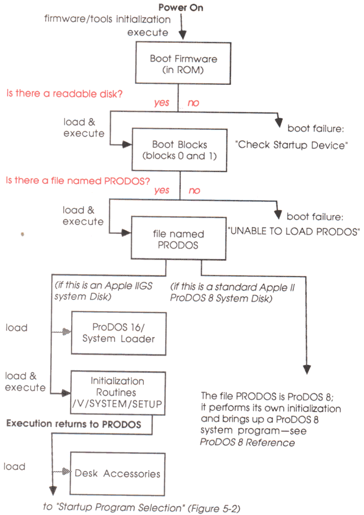
Figure 5-1 Boot initialization sequence
