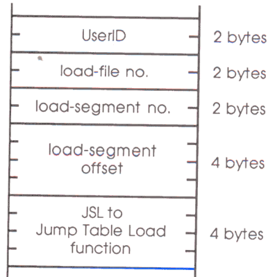
Figure 15-3 Jump Table entry (unloaded state)
