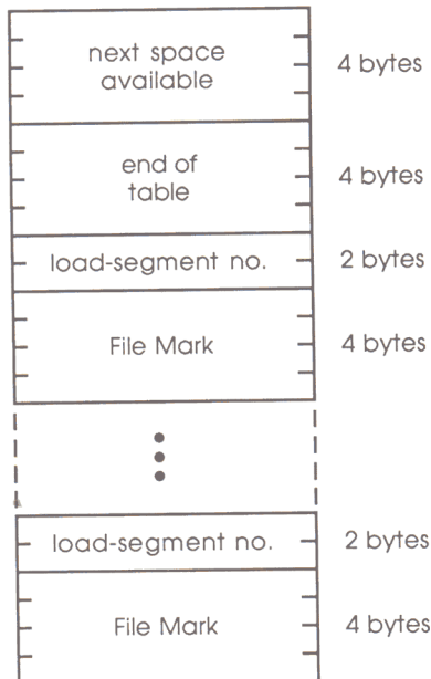
Figure 15-7 Mark List format
