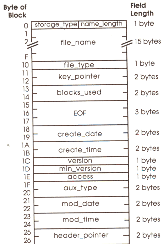
Figure A-5 The file entry
