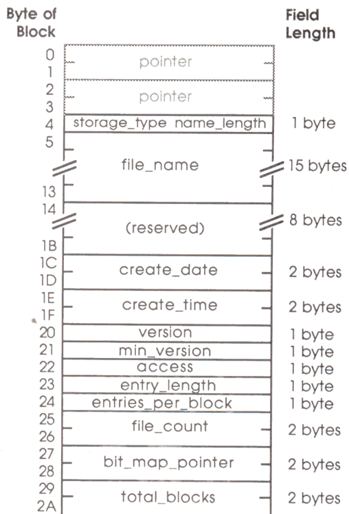
Figure A-3 The volume directory header
