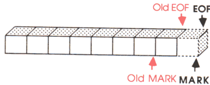
Figure 2-2 Automatic movement of EOF and Mark
