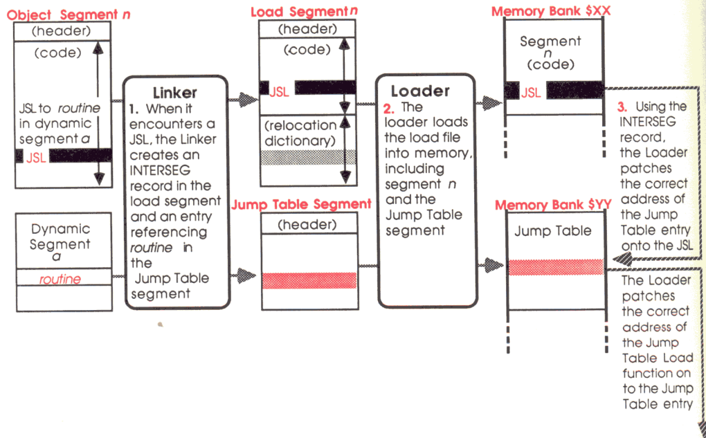
Figure 15-5A How the Jump Table works
