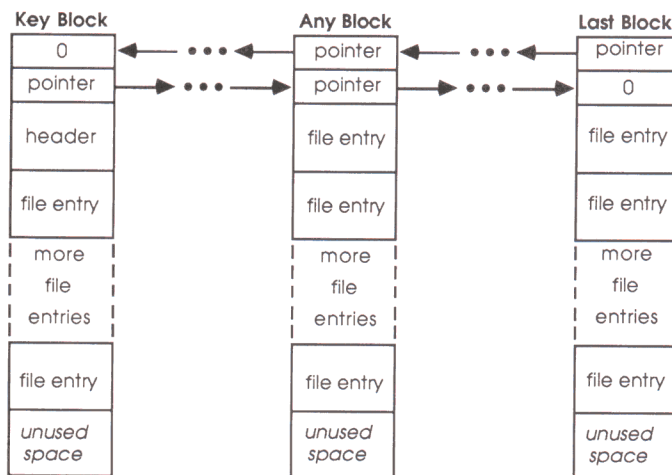
Figure A-2 Directory file format and organization
