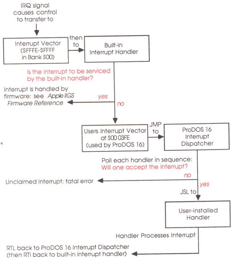
Figure 4-1 Interrupt handling through ProDOS 16
